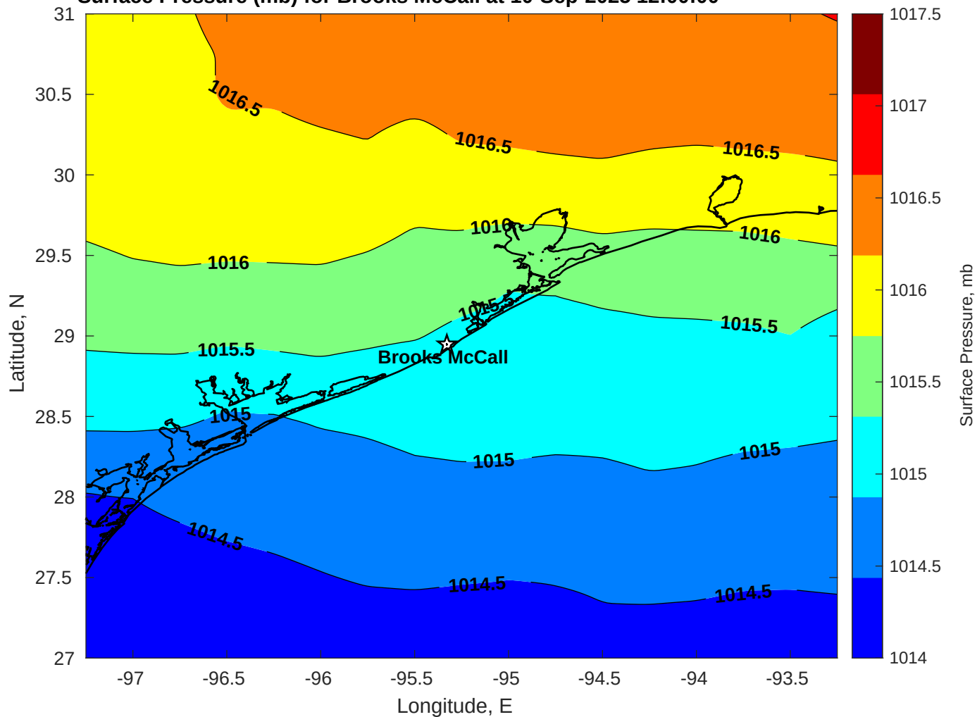
Surface Pressure (mb) for Brooks McCall at 10-Sep-2025 12:00:00
