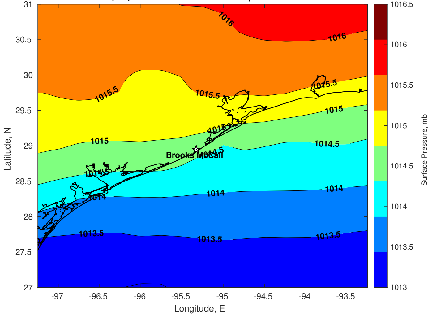
Surface Pressure (mb) for Brooks McCall at 09-Sep-2025 12:00:00
