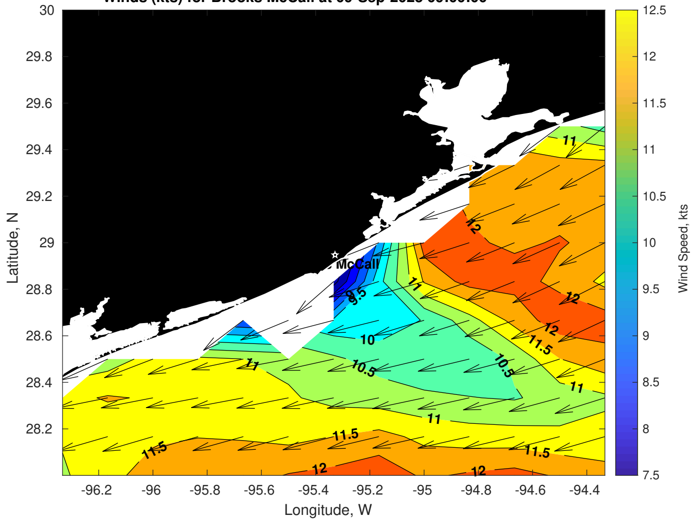
Winds (kts) for Brooks McCall at 09-Sep-2025 09:00:00
