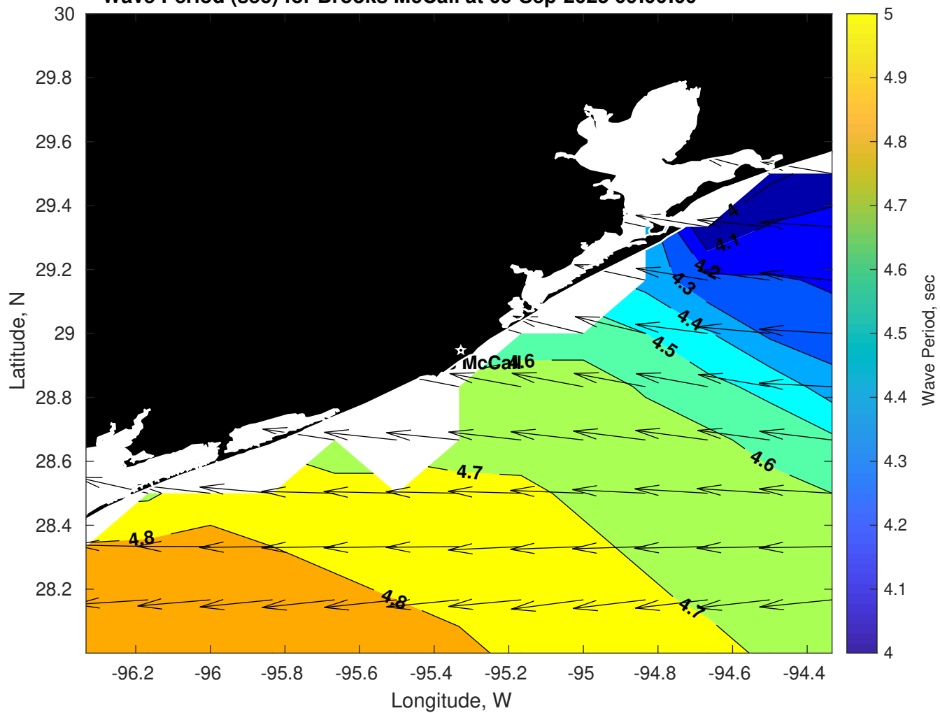
Wave Period (sec) for Brooks McCall at 09-Sep-2025 09:00:00
