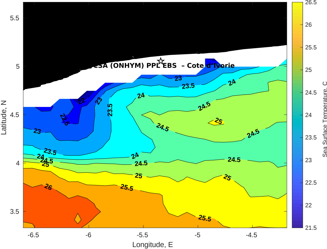
SST for CSA (ONHYM) PPL EBS - Cote d'Ivoire at 08-Sep-2025 00:00:00
