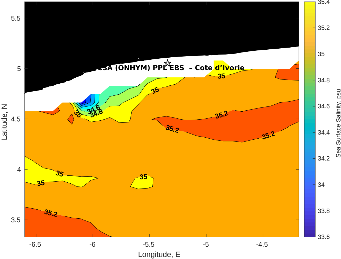
Surface Salinity for CSA (ONHYM) PPL EBS - Cote d'Ivoire at 08-Sep-2025 00:00:00
