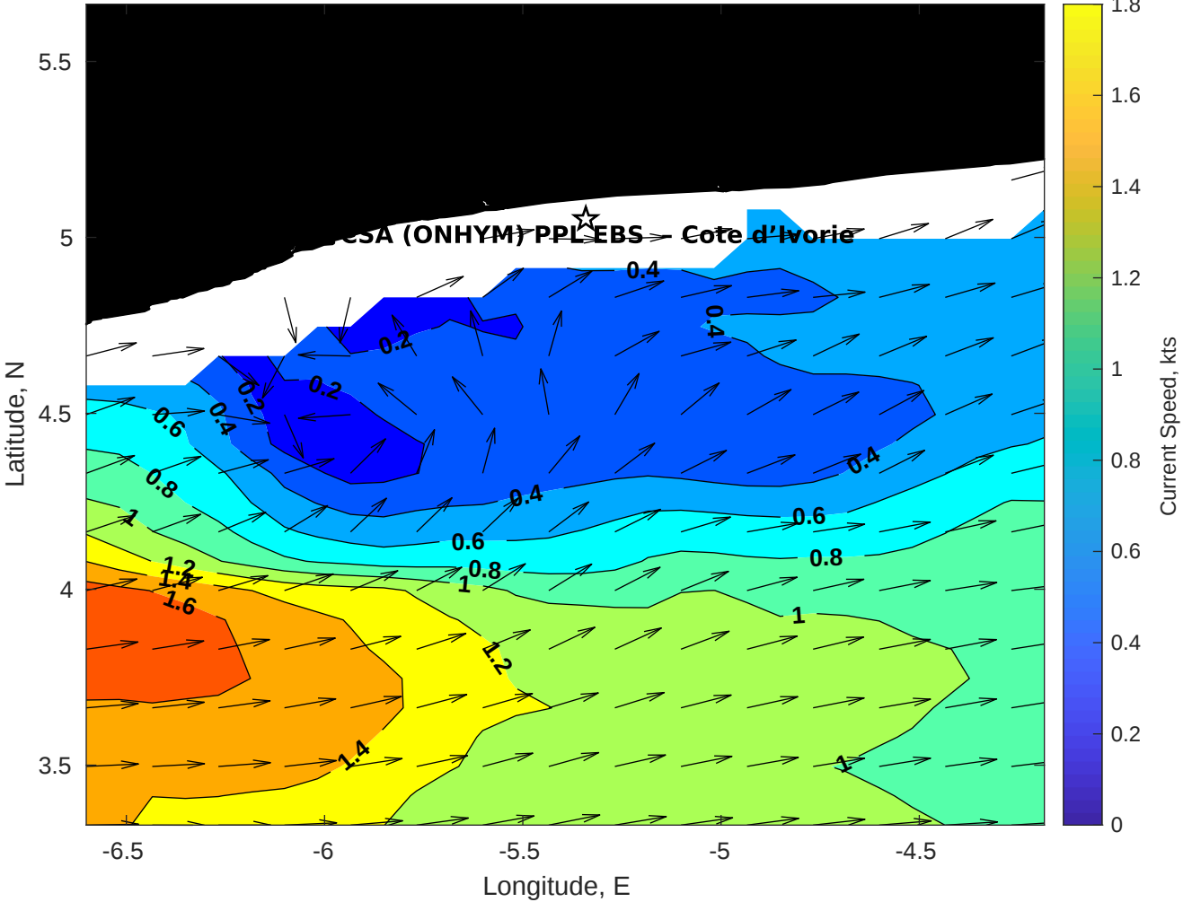
Surface Currents for CSA (ONHYM) PPL EBS - Cote d'Ivoire at 08-Sep-2025 00:00:00
