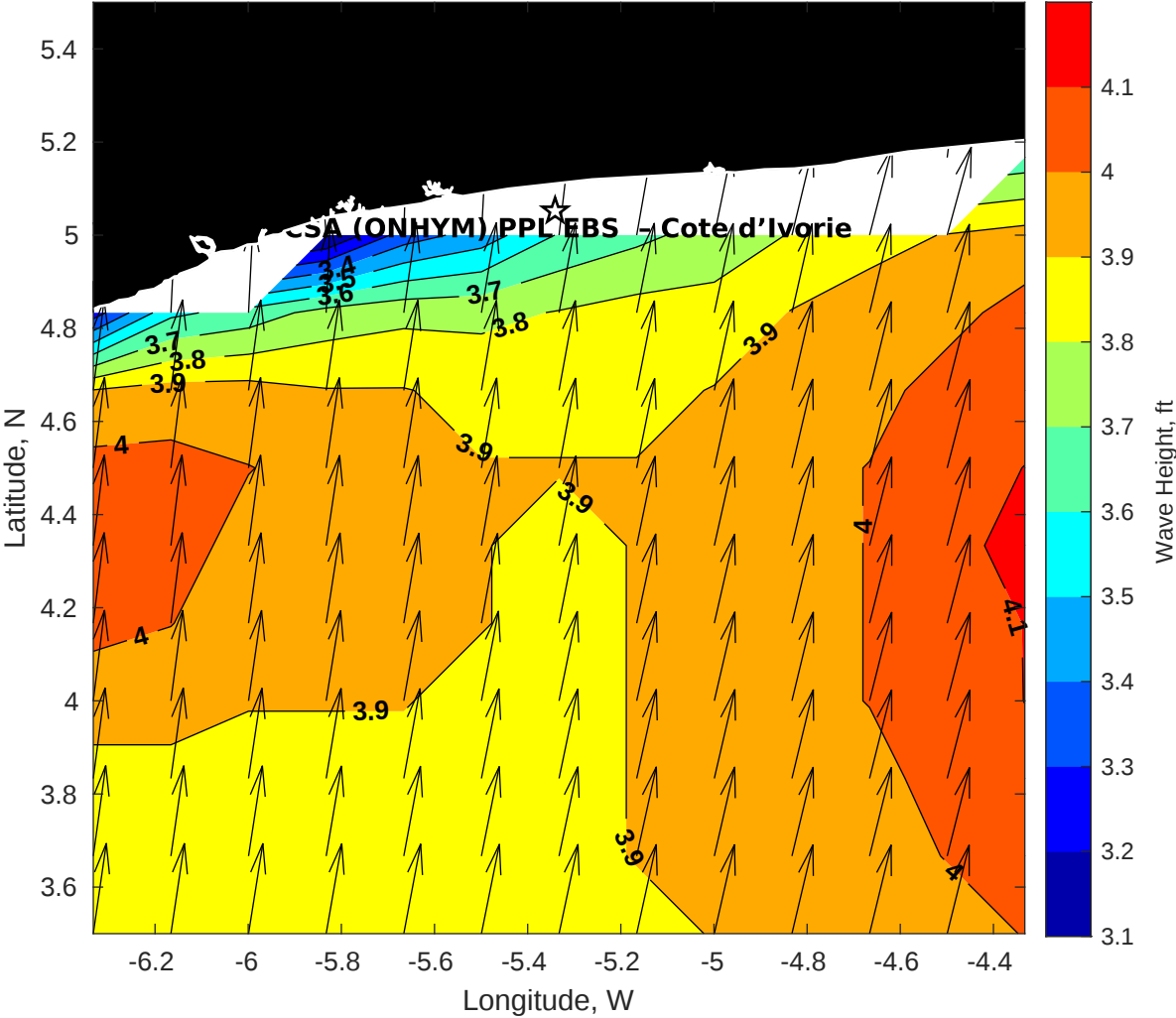
Wave Height (ft) for CSA (ONHYM) PPL EBS - Cote d'Ivoire at 09-Sep-2025 09:00:00
