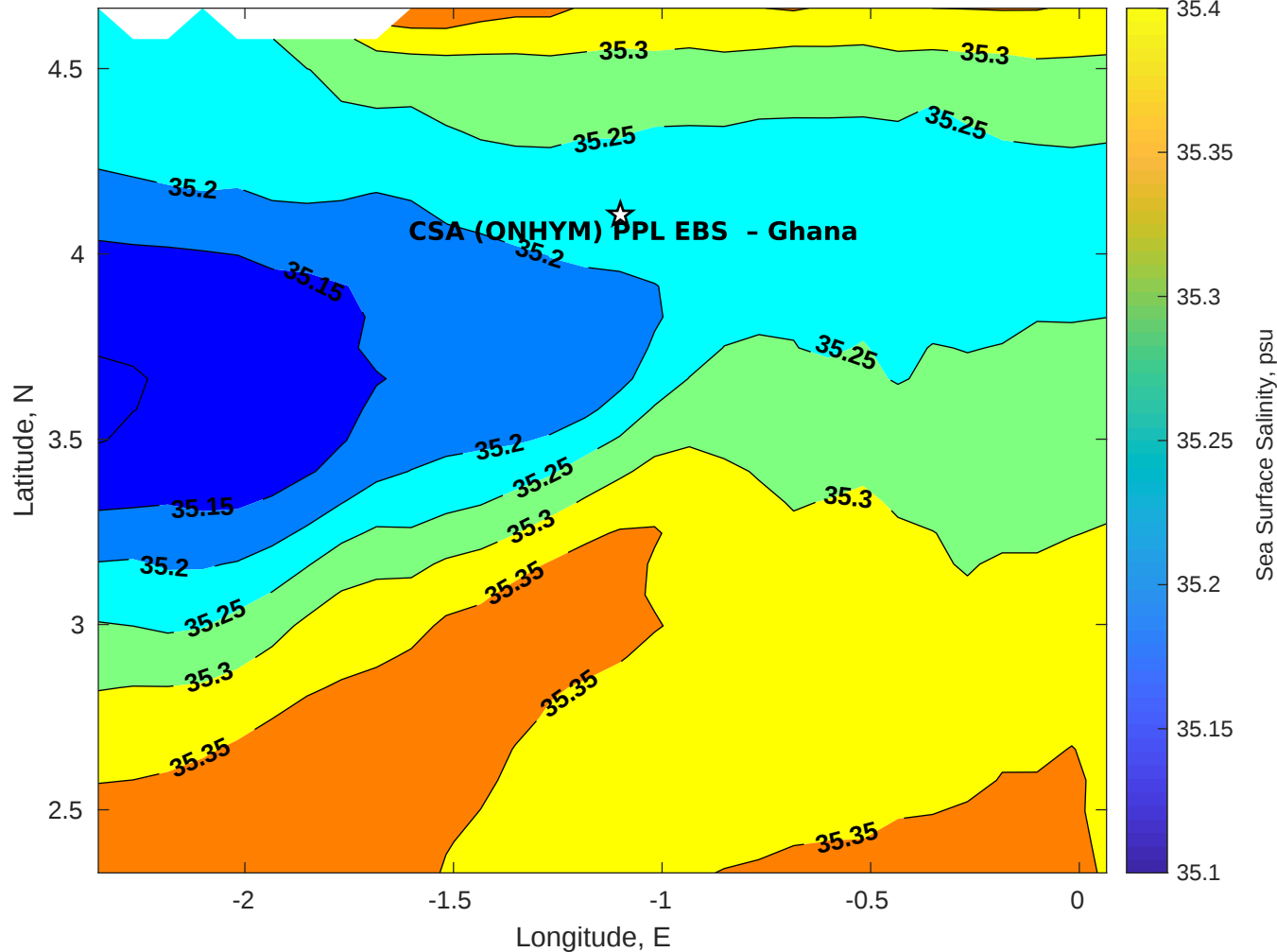
Surface Salinity for CSA (ONHYM) PPL EBS - Ghana at 08-Sep-2025 00:00:00
