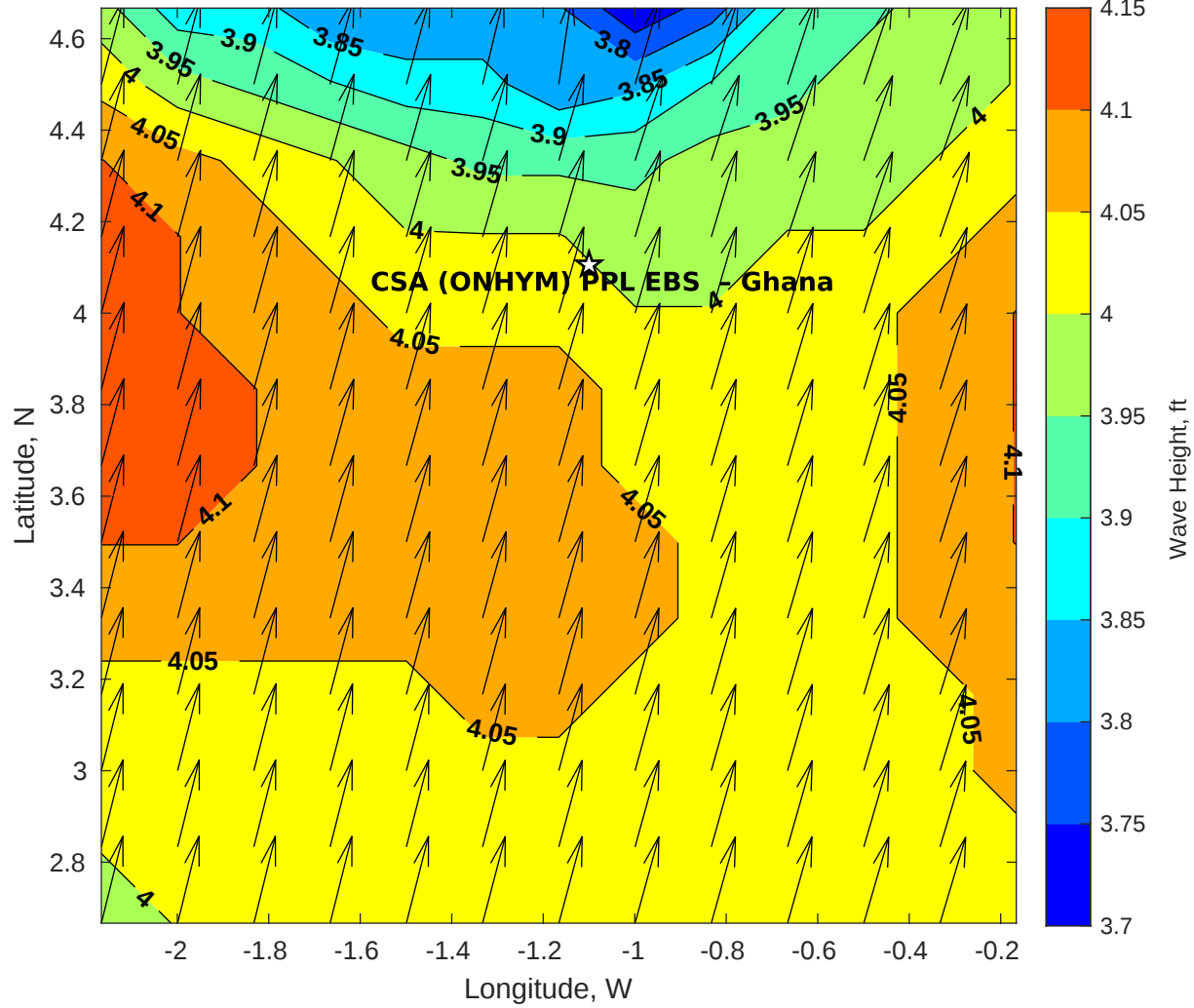
Wave Height (ft) for CSA (ONHYM) PPL EBS - Ghana at 09-Sep-2025 09:00:00
