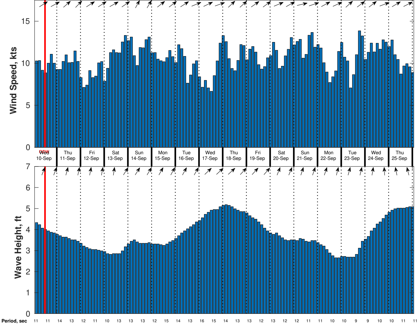
Wind & Wave Forecast for CSA (ONHYM) PPL EBS - Ghana from 09-Sep-2025 02:00:00 to 25-Sep-2025 02:00:00
