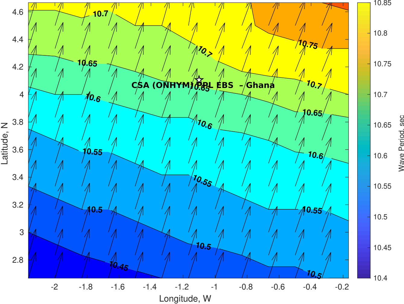
Wave Period (sec) for CSA (ONHYM) PPL EBS - Ghana at 09-Sep-2025 09:00:00
