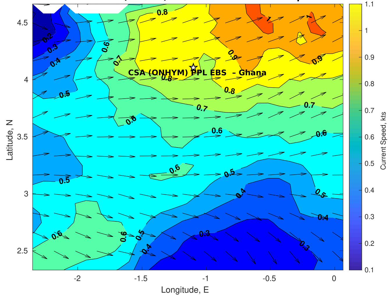
Surface Currents for CSA (ONHYM) PPL EBS - Ghana at 08-Sep-2025 00:00:00
