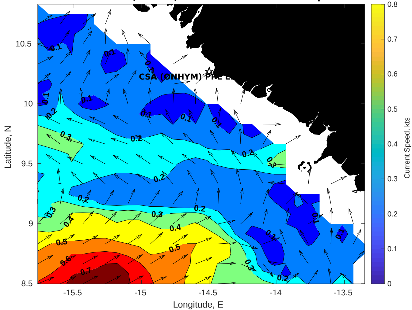
Surface Currents for CSA (ONHYM) PPL EBS - Guinea at 08-Sep-2025 00:00:00
