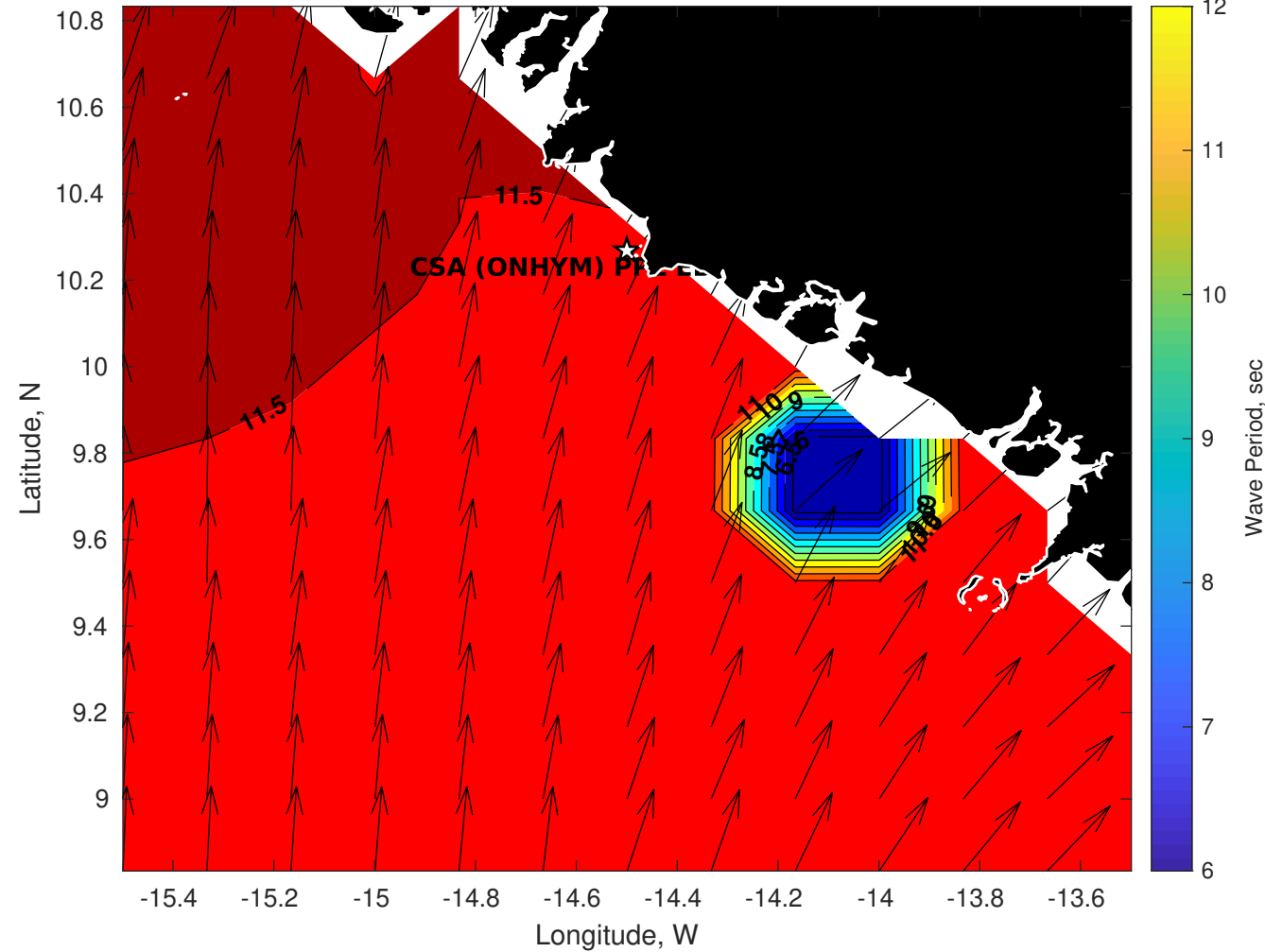
Wave Period (sec) for CSA (ONHYM) PPL EBS - Guinea at 09-Sep-2025 09:00:00
