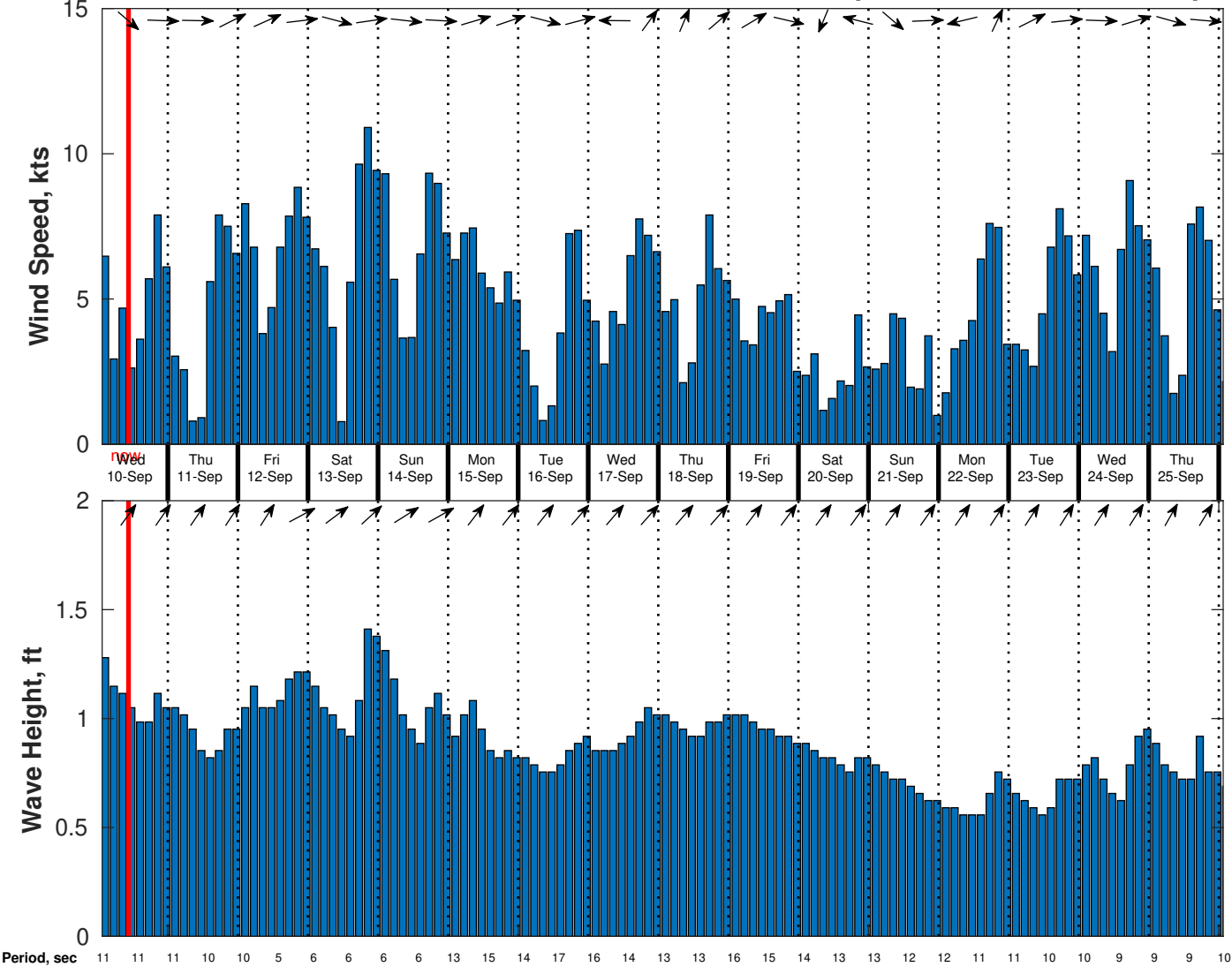
Wind & Wave Forecast for CSA (ONHYM) PPL EBS - Guinea from 09-Sep-2025 01:00:00 to 25-Sep-2025 01:00:00
