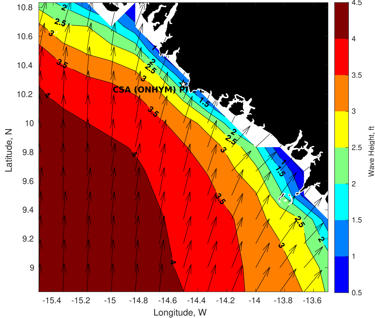
Wave Height (ft) for CSA (ONHYM) PPL EBS - Guinea at 09-Sep-2025 09:00:00
