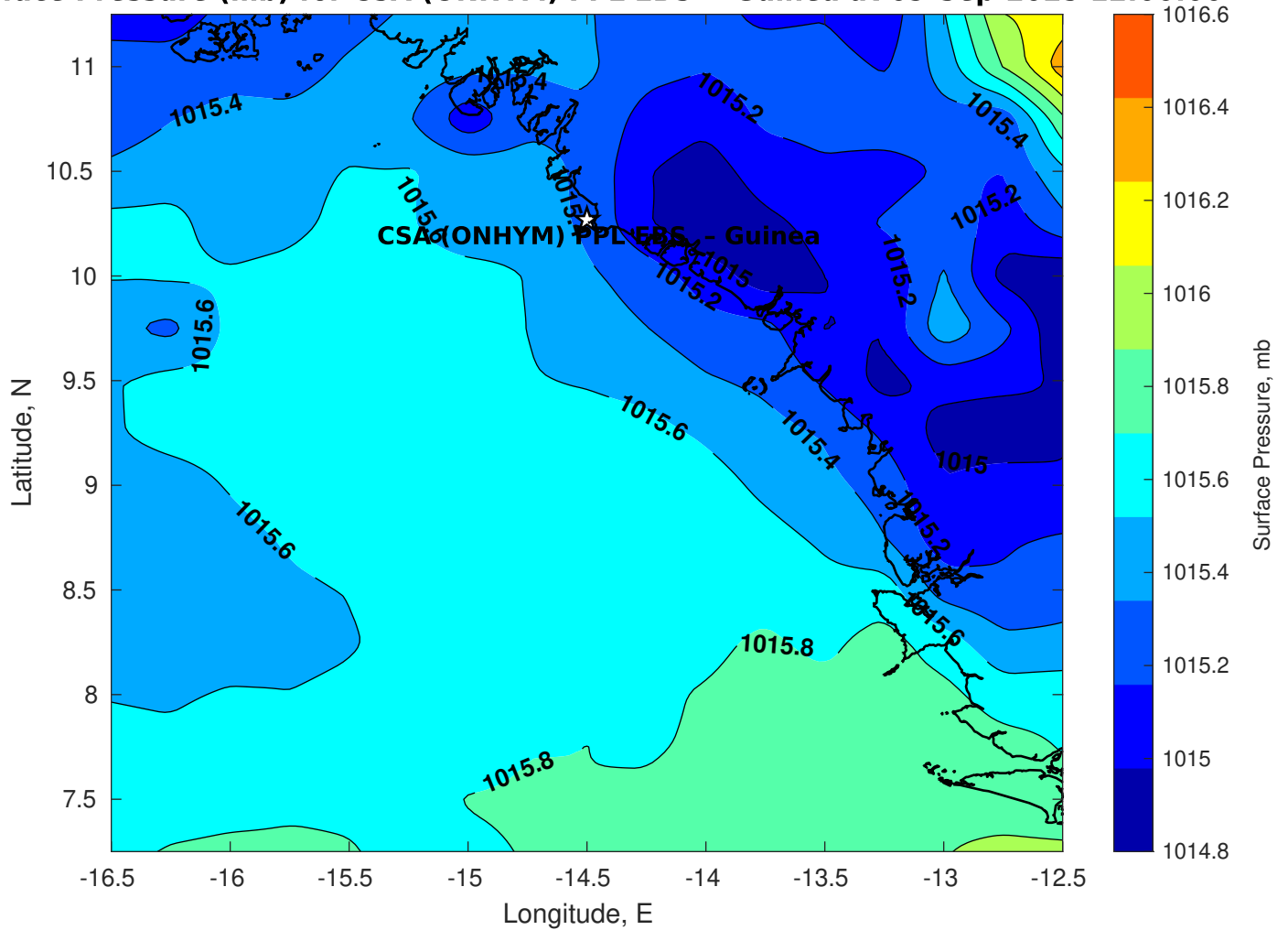
Surface Pressure (mb) for CSA (ONHYM) PPL EBS - Guinea at 09-Sep-2025 12:00:00
