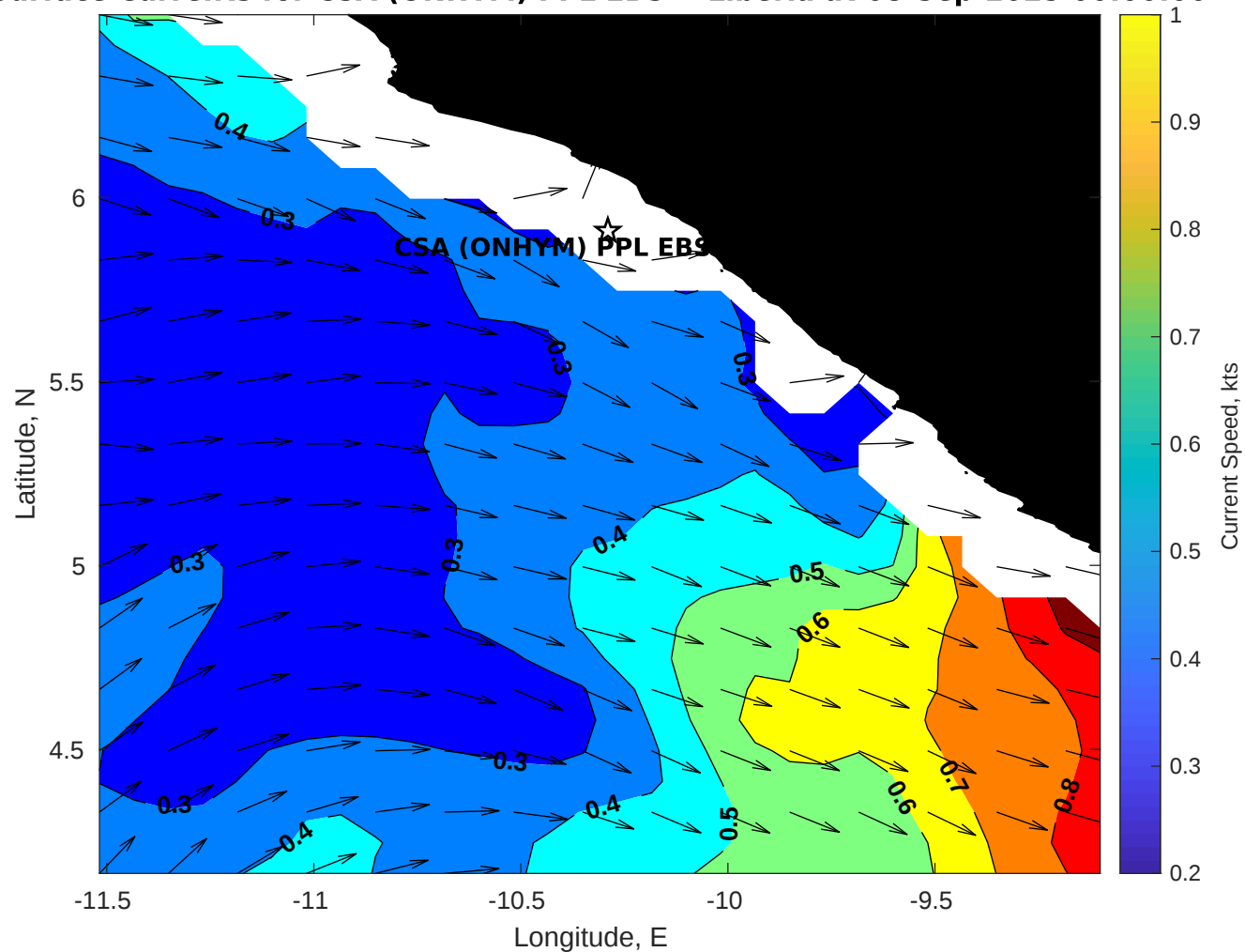
Surface Currents for CSA (ONHYM) PPL EBS - Liberia at 08-Sep-2025 00:00:00
