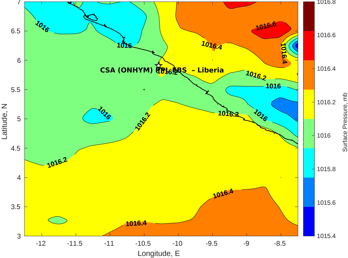
Surface Pressure (mb) for CSA (ONHYM) PPL EBS - Liberia at 09-Sep-2025 12:00:00
