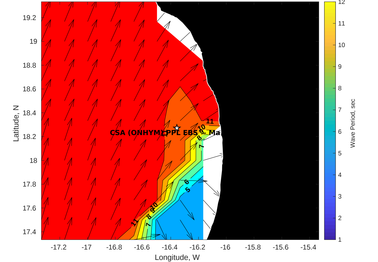
Wave Period (sec) for CSA (ONHYM) PPL EBS - Mauritania at 09-Sep-2025 09:00:00
