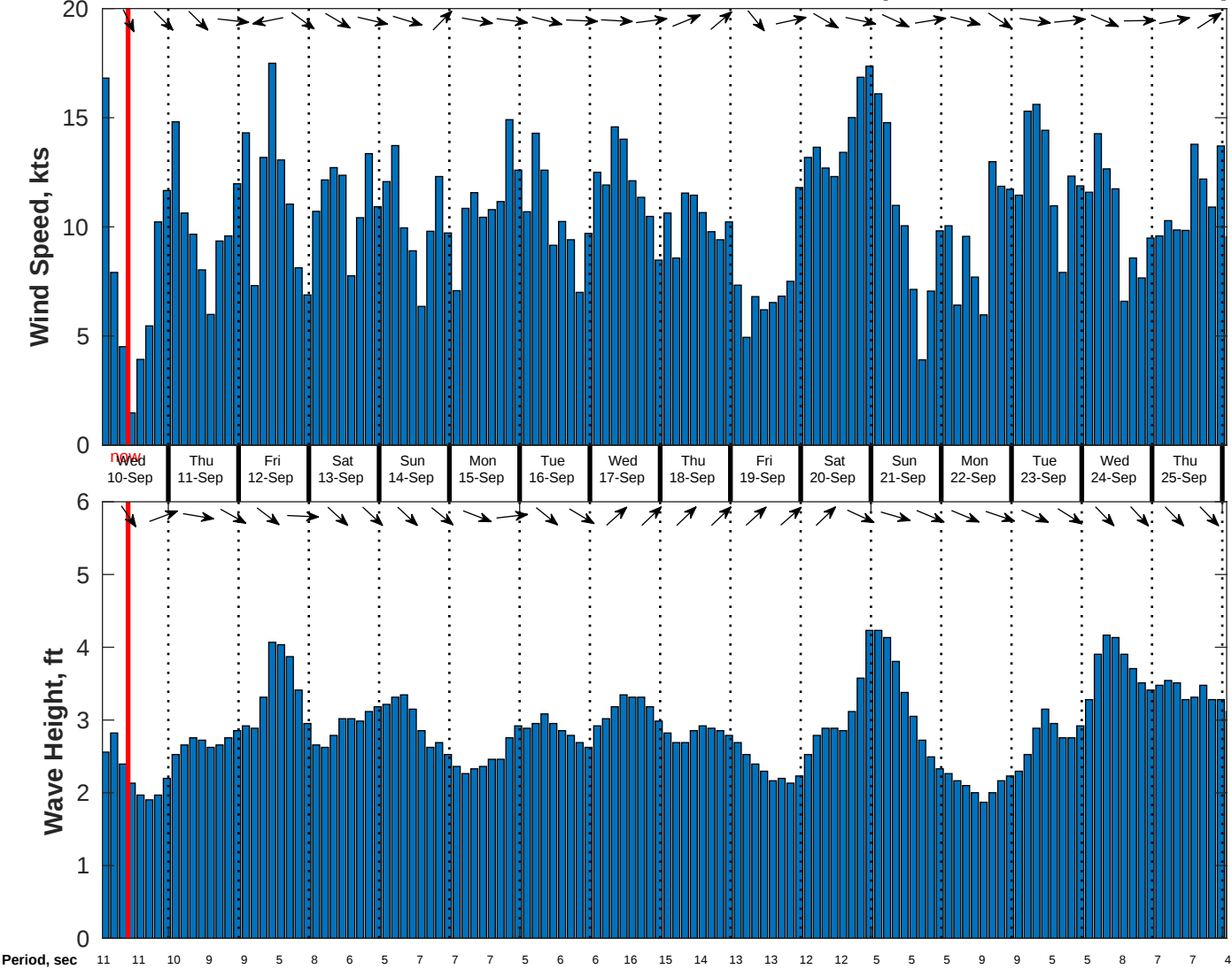
Wind & Wave Forecast for CSA (ONHYM) PPL EBS - Mauritania from 09-Sep-2025 01:00:00 to 25-Sep-2025 01:00:00
