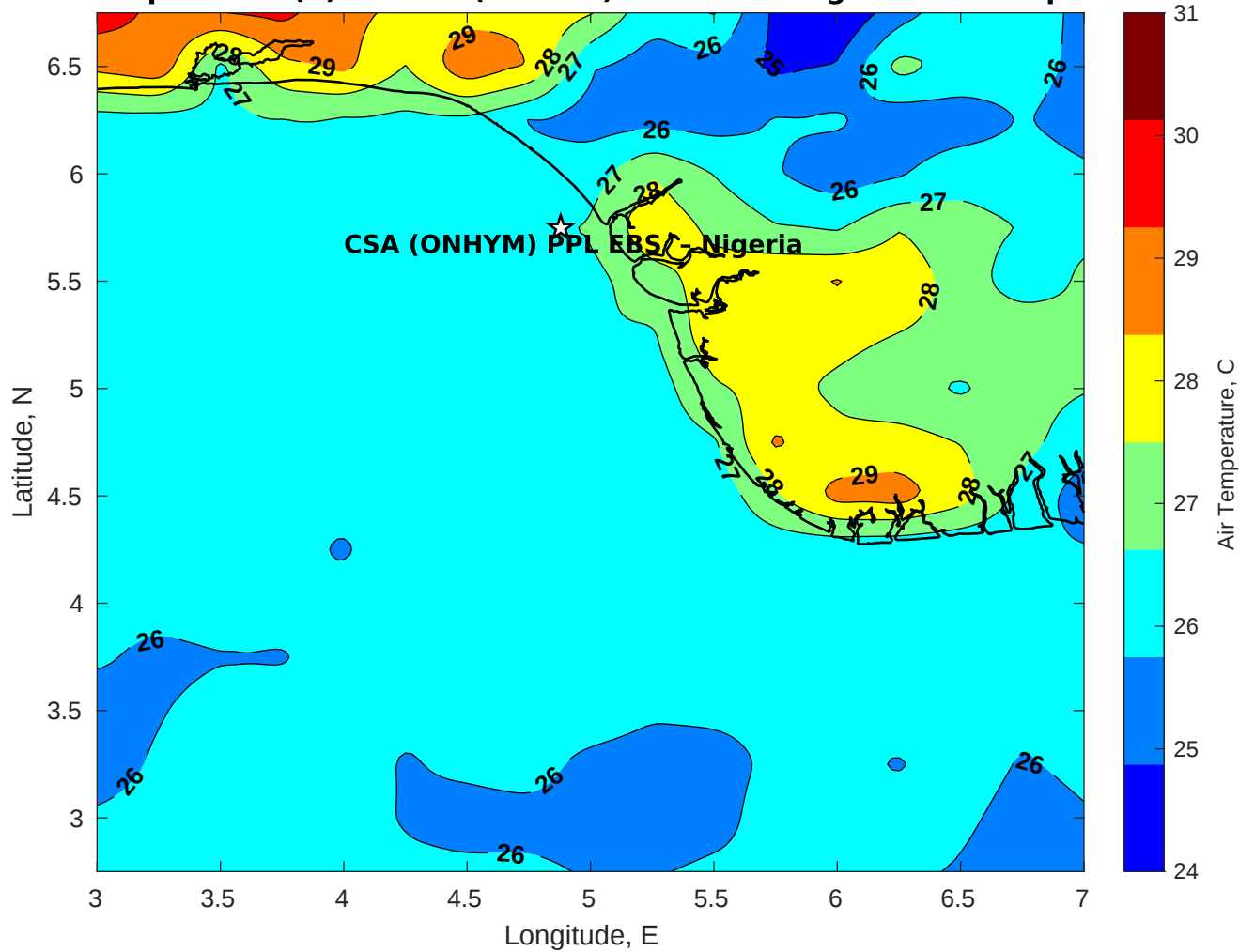
Air Temperature (C) for CSA (ONHYM) PPL EBS - Nigeria at 08-Sep-2025
