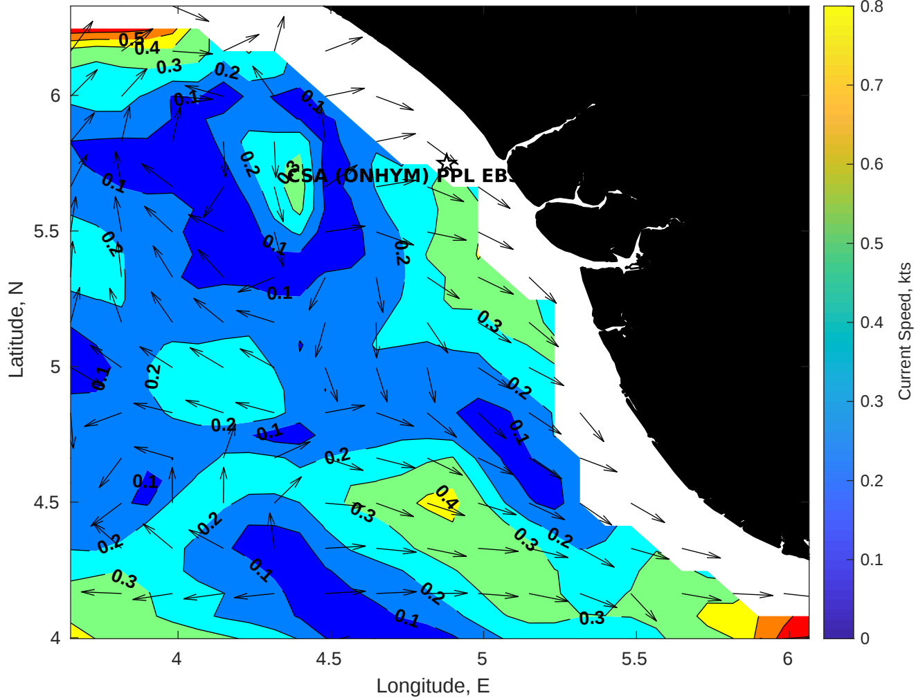
Surface Currents for CSA (ONHYM) PPL EBS - Nigeria at 08-Sep-2025 00:00:00
