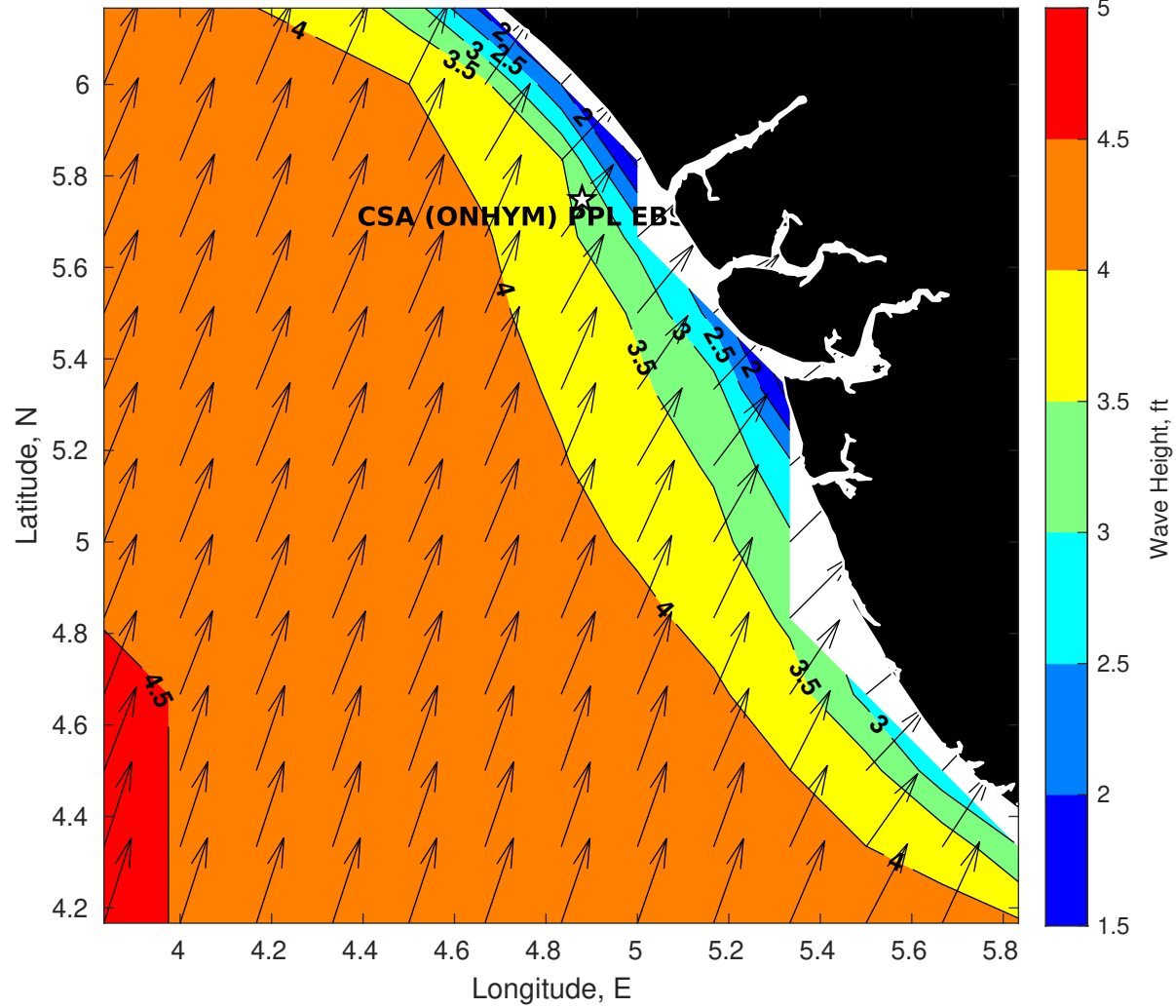
Wave Height (ft) for CSA (ONHYM) PPL EBS - Nigeria at 09-Sep-2025 09:00:00
