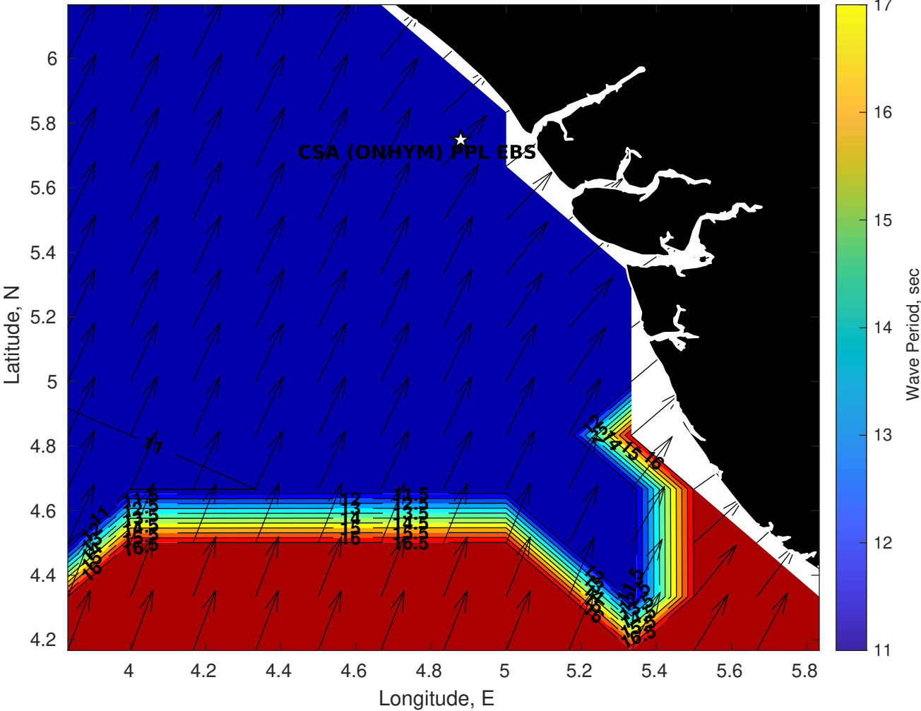
Wave Period (sec) for CSA (ONHYM) PPL EBS - Nigeria at 09-Sep-2025 09:00:00
