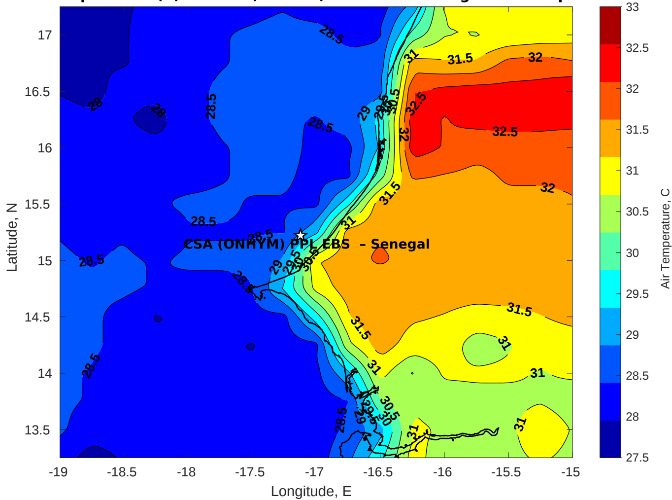
Air Temperature (C) for CSA (ONHYM) PPL EBS - Senegal at 08-Sep-2025
