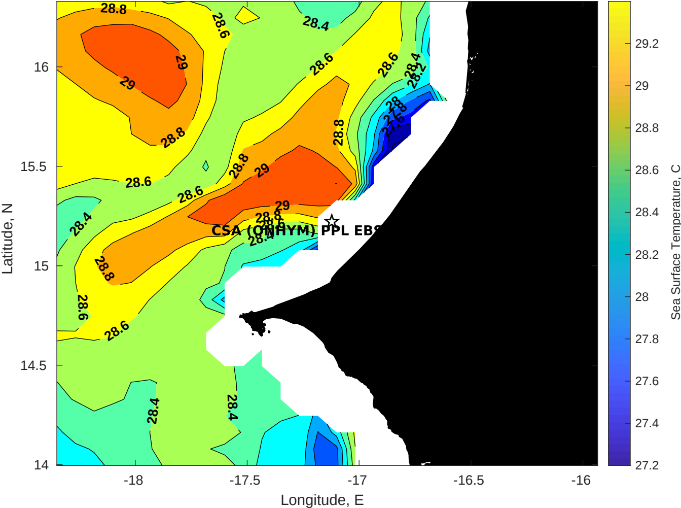
SST for CSA (ONHYM) PPL EBS - Senegal at 08-Sep-2025 00:00:00
