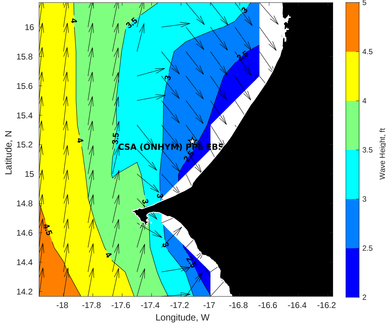
Wave Height (ft) for CSA (ONHYM) PPL EBS - Senegal at 09-Sep-2025 09:00:00
