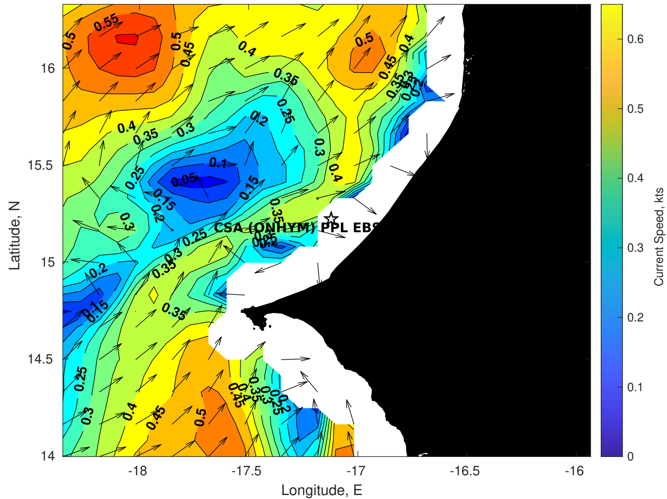
Surface Currents for CSA (ONHYM) PPL EBS - Senegal at 08-Sep-2025 00:00:00
