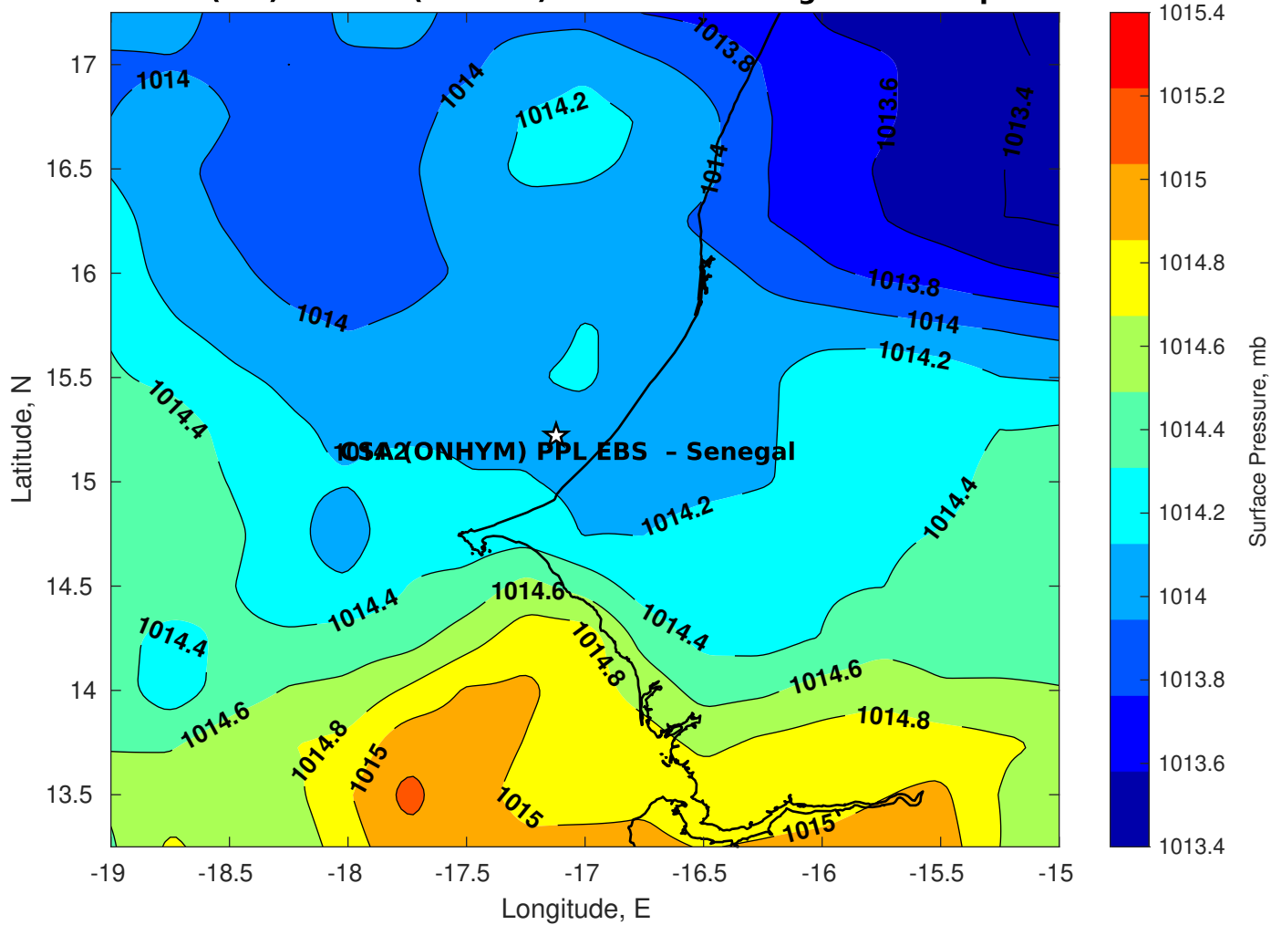
Surface Pressure (mb) for CSA (ONHYM) PPL EBS - Senegal at 09-Sep-2025 12:00:00
