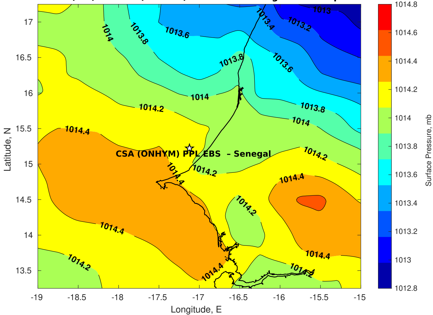
Surface Pressure (mb) for CSA (ONHYM) PPL EBS - Senegal at 10-Sep-2025 12:00:00
