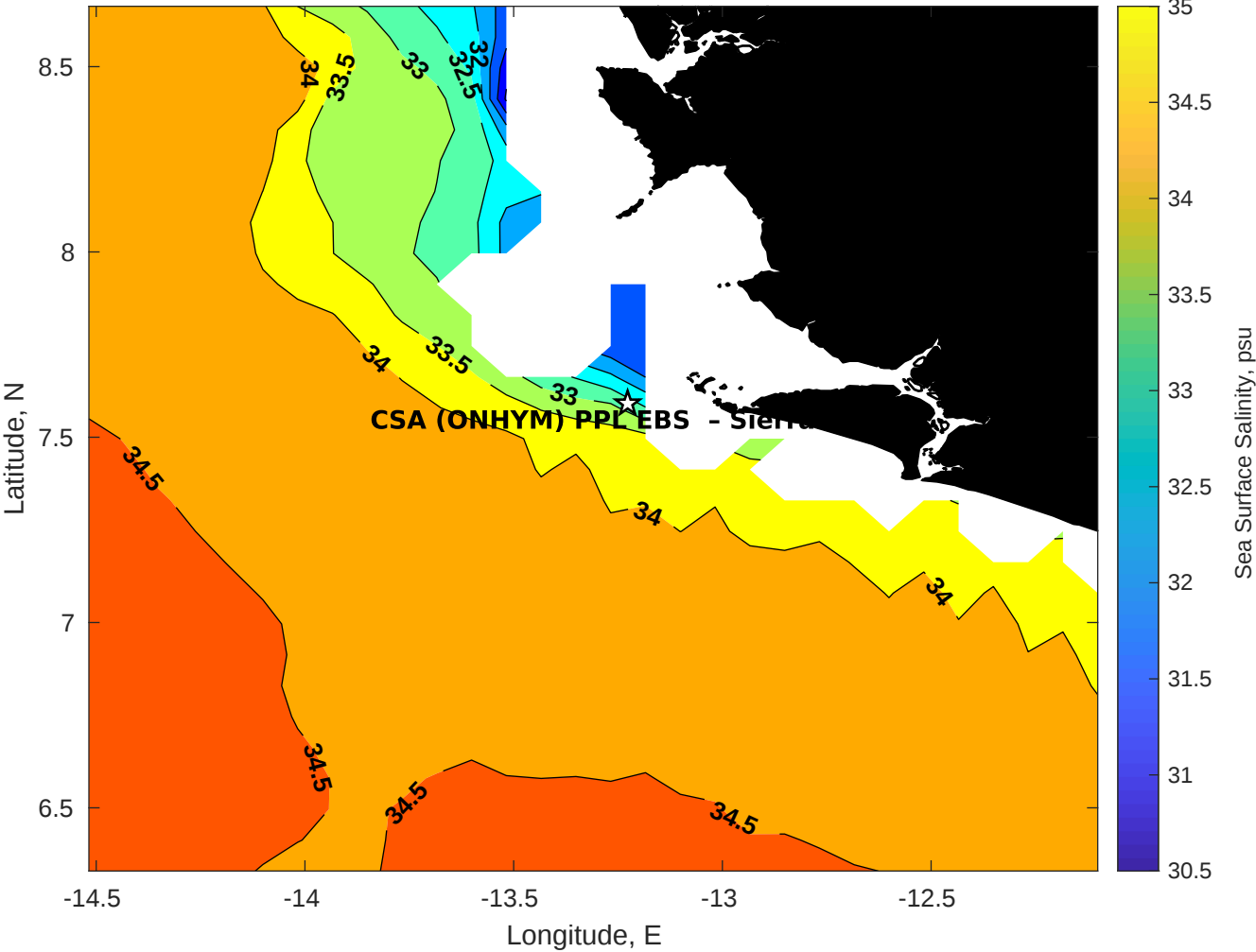
Surface Salinity for CSA (ONHYM) PPL EBS - Sierra Leone at 08-Sep-2025 00:00:00
