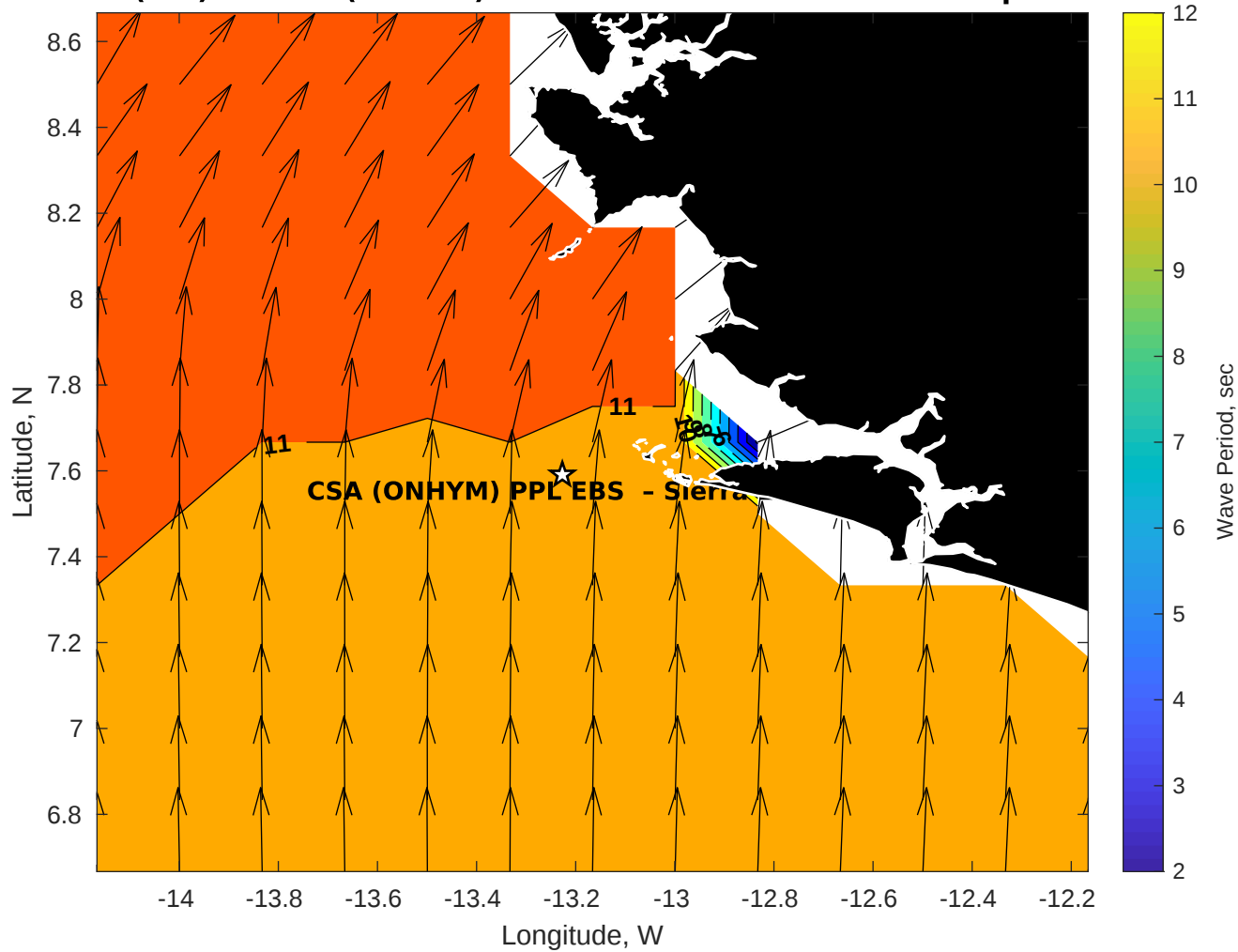
Wave Period (sec) for CSA (ONHYM) PPL EBS - Sierra Leone at 09-Sep-2025 09:00:00
