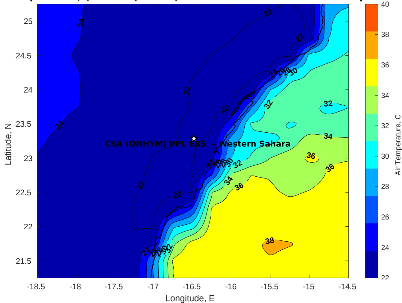
Air Temperature (C) for CSA (ONHYM) PPL EBS - Western Sahara at 08-Sep-2025
