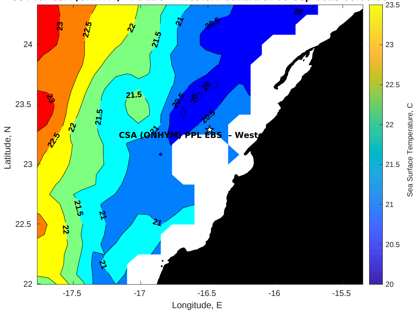
SST for CSA (ONHYM) PPL EBS - Western Sahara at 08-Sep-2025 00:00:00
