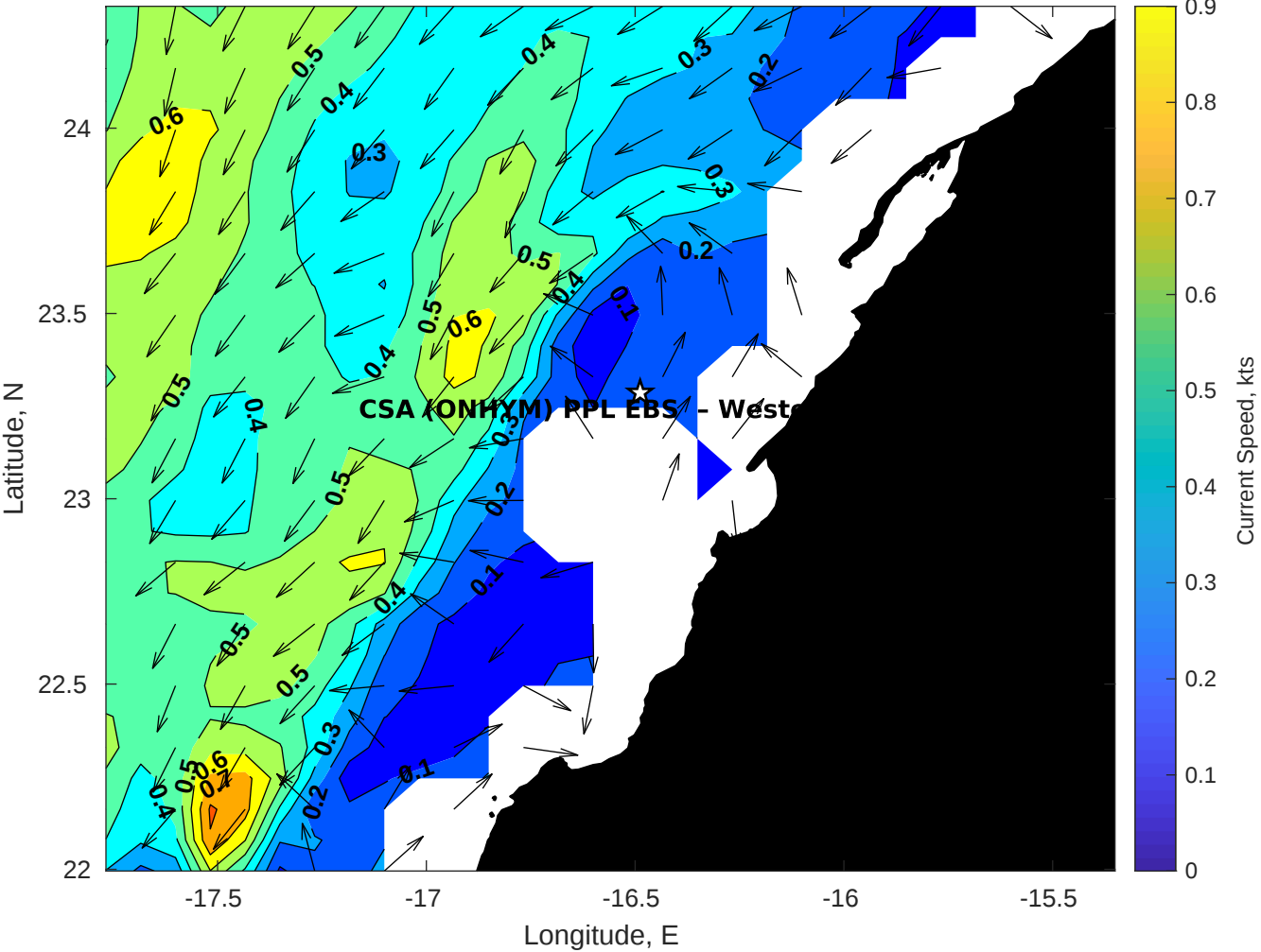
Surface Currents for CSA (ONHYM) PPL EBS - Western Sahara at 08-Sep-2025 00:00:00
