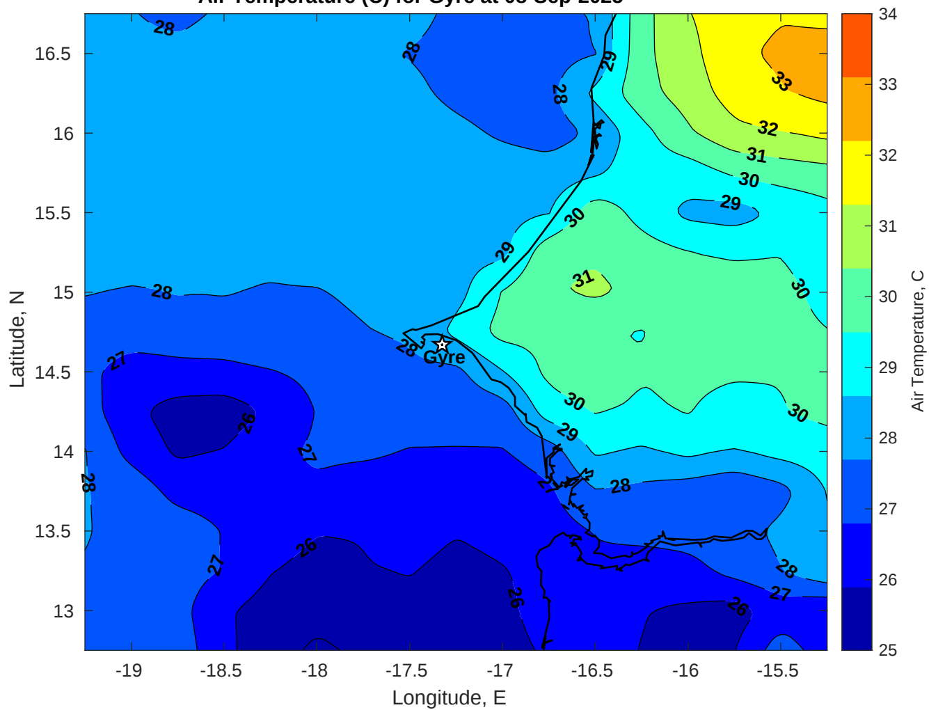
Air Temperature (C) for Gyre at 08-Sep-2025
