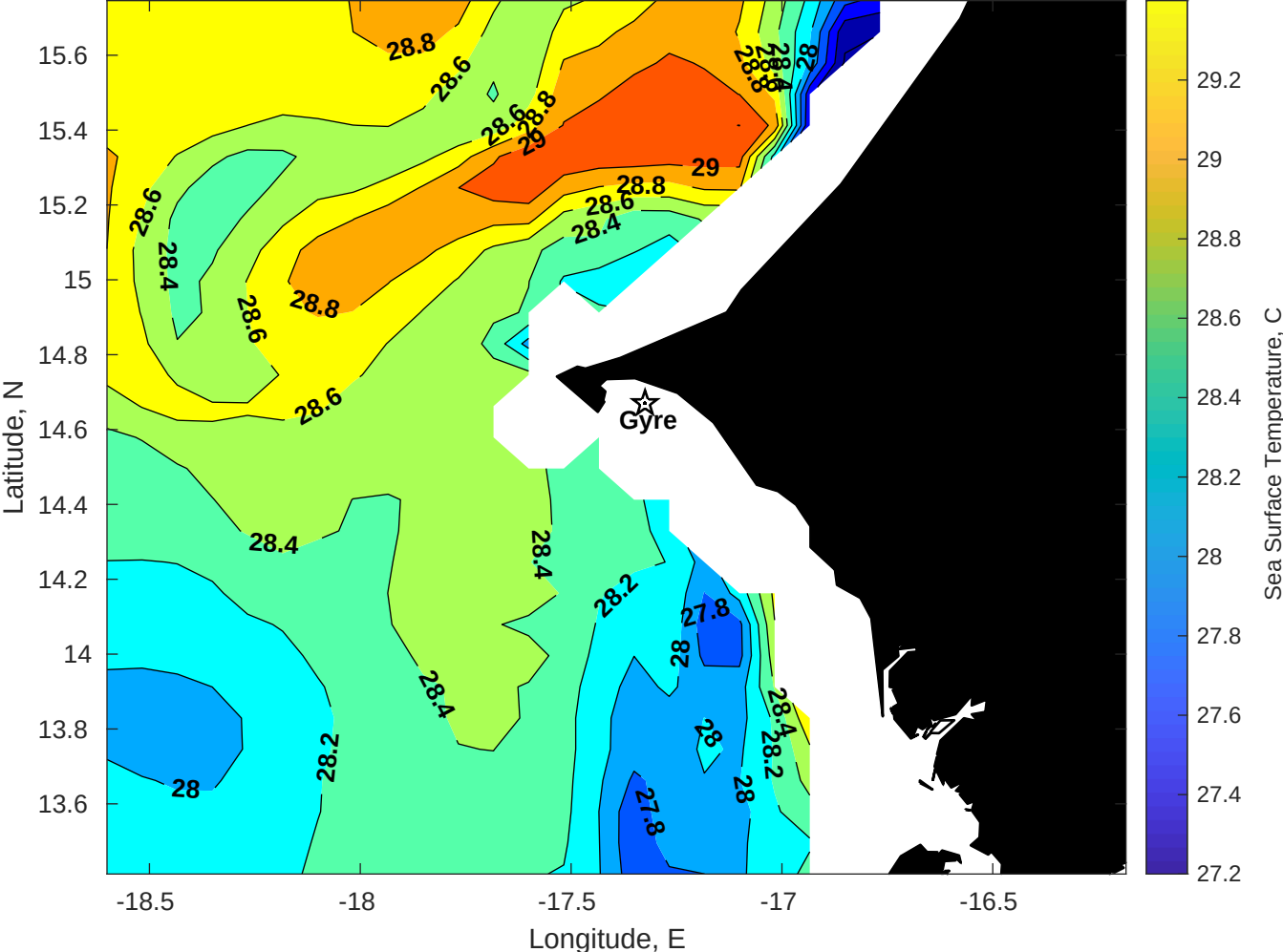
SST for Gyre at 08-Sep-2025 00:00:00
