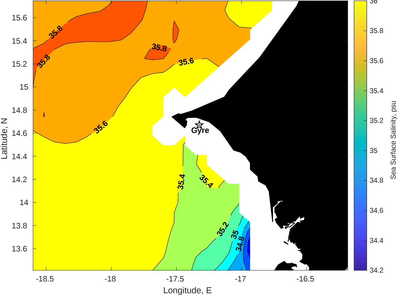
Surface Salinity for Gyre at 08-Sep-2025 00:00:00
