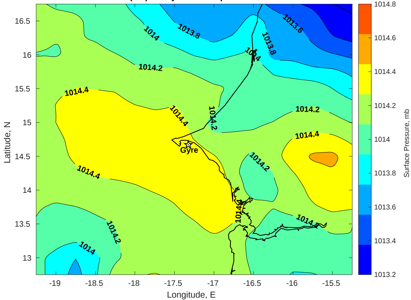
Surface Pressure (mb) for Gyre at 10-Sep-2025 12:00:00
