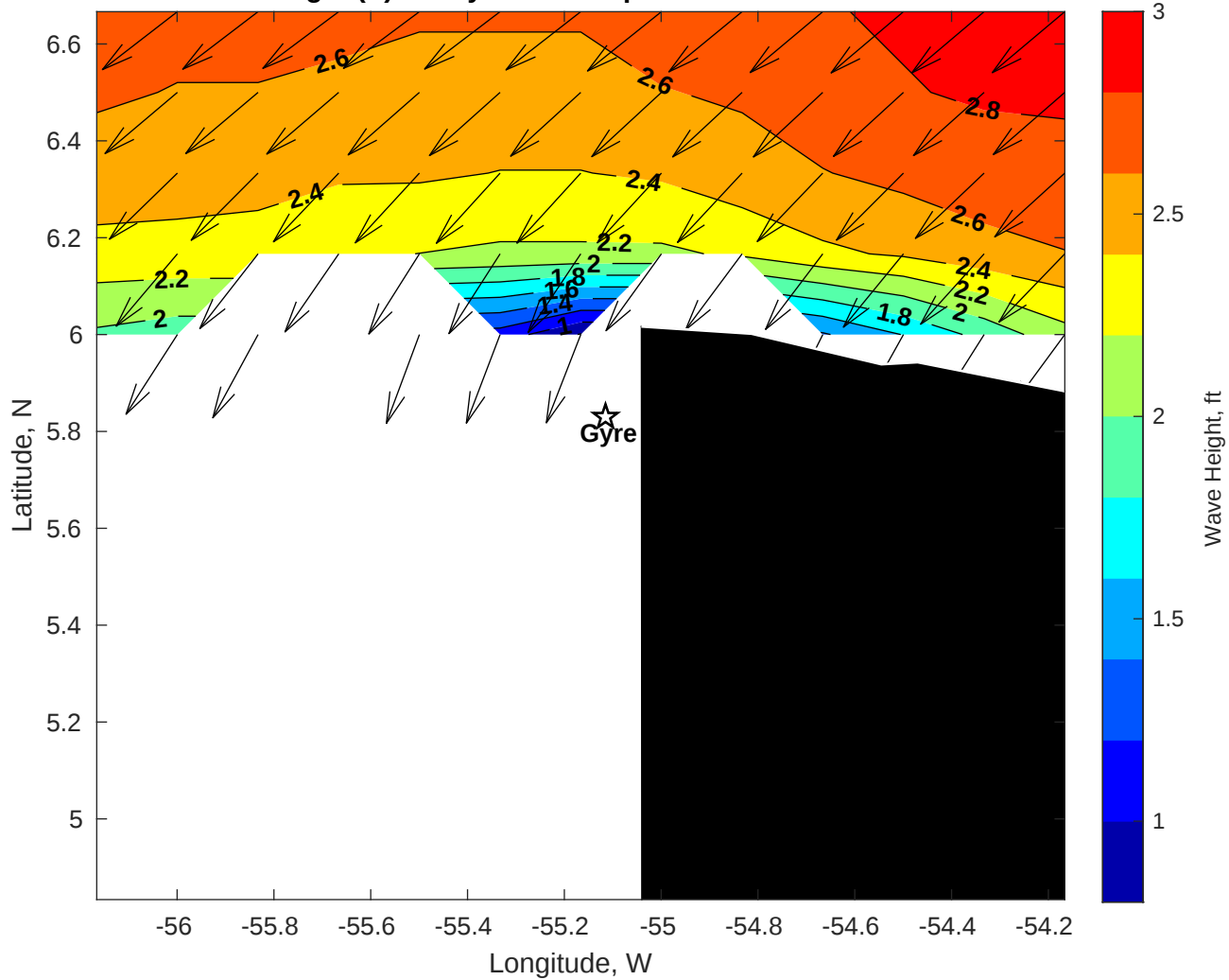
Wave Height (ft) for Gyre at 09-Sep-2025 09:00:00
