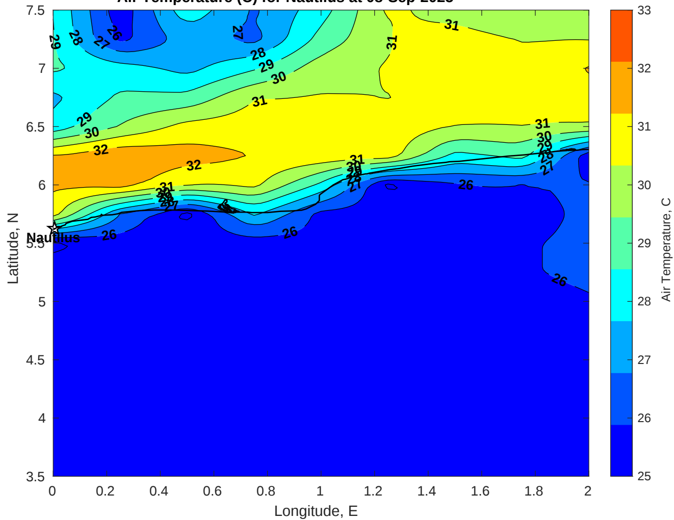
Air Temperature (C) for Nautilus at 08-Sep-2025
