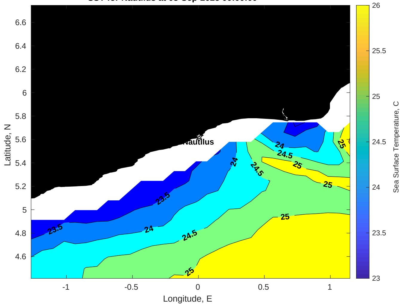
SST for Nautilus at 08-Sep-2025 00:00:00
