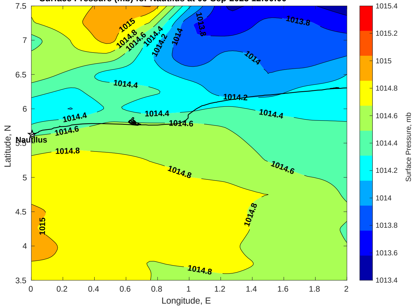
Surface Pressure (mb) for Nautilus at 09-Sep-2025 12:00:00
