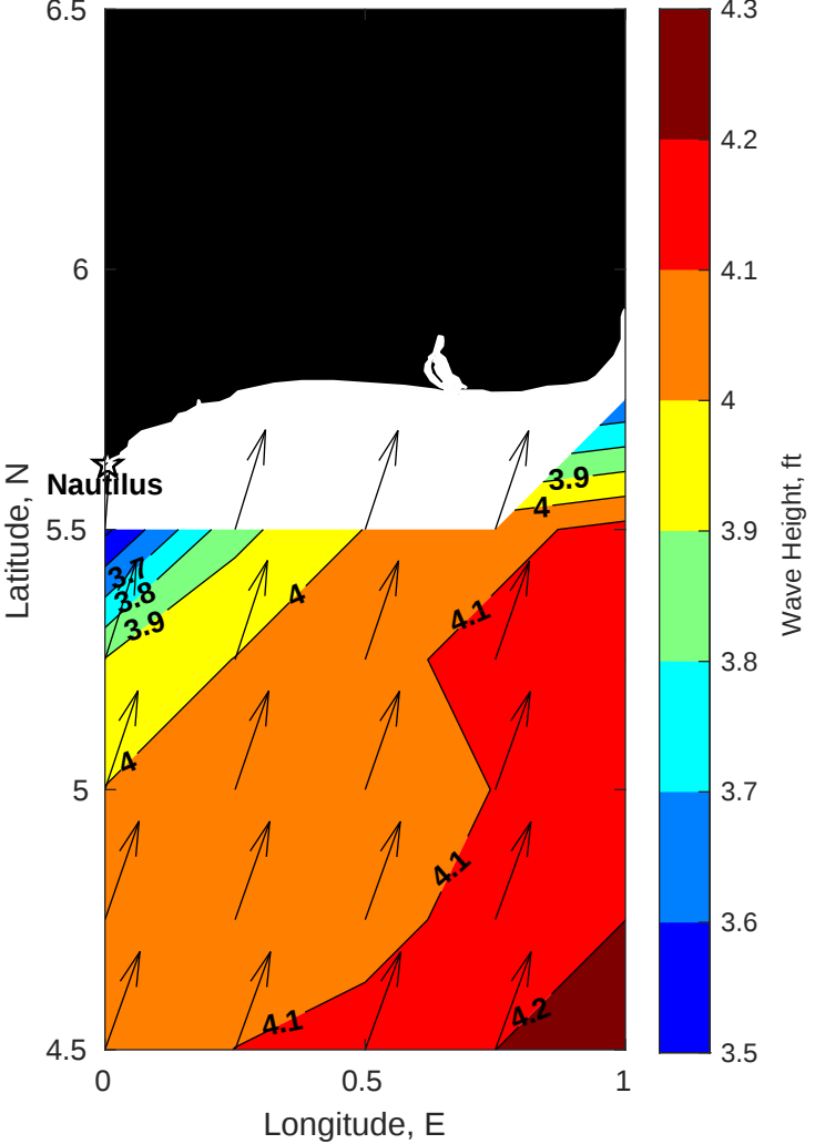
Wave Height (ft) for Nautilus at 09-Sep-2025 09:00:00
