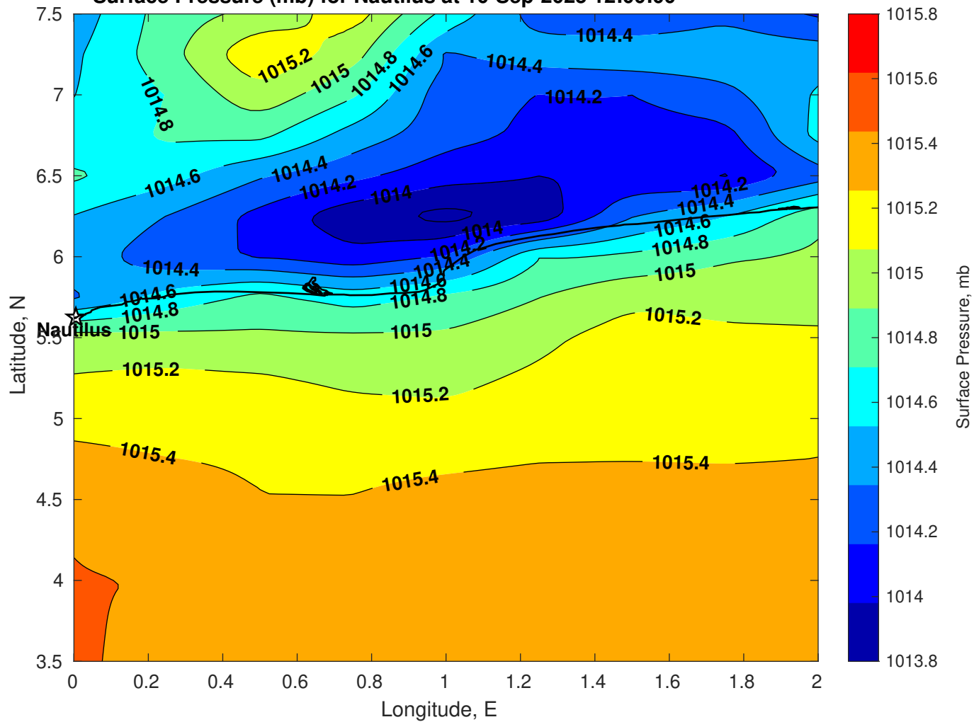
Surface Pressure (mb) for Nautilus at 10-Sep-2025 12:00:00
