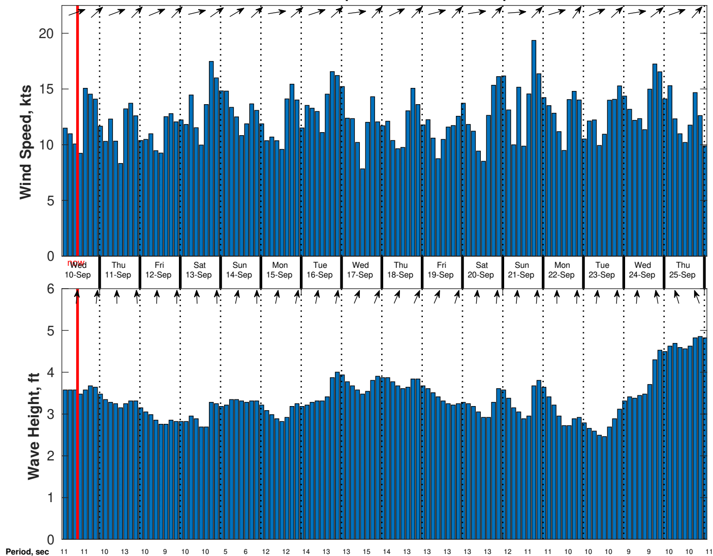
Wind & Wave Forecast for Nautilus from 09-Sep-2025 02:00:00 to 25-Sep-2025 02:00:00
