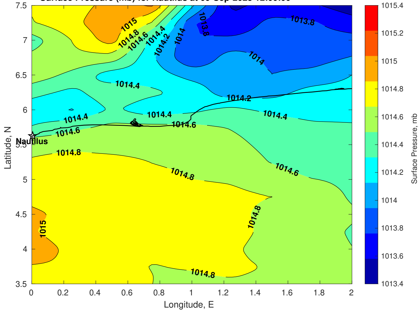
Surface Pressure (mb) for Nautilus at 09-Sep-2025 12:00:00
