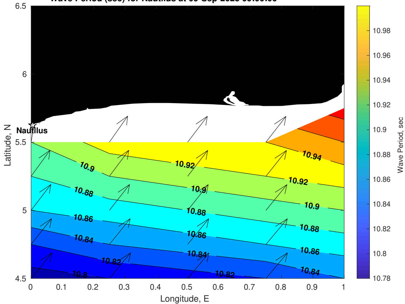
Wave Period (sec) for Nautilus at 09-Sep-2025 09:00:00
