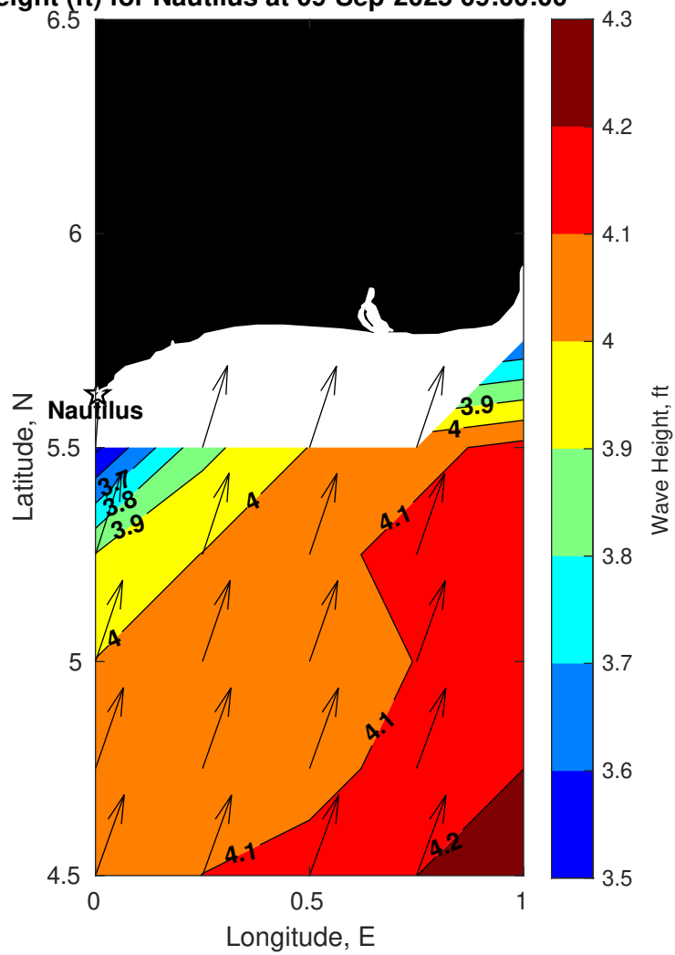
Wave Height (ft) for Nautilus at 09-Sep-2025 09:00:00
