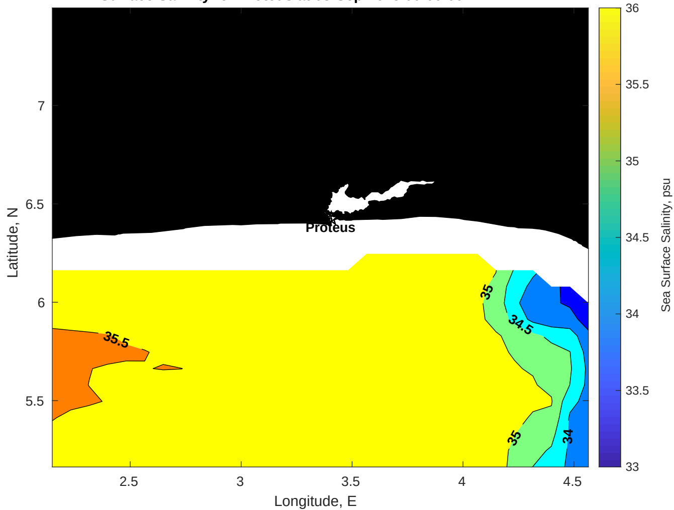
Surface Salinity for Proteus at 08-Sep-2025 00:00:00
