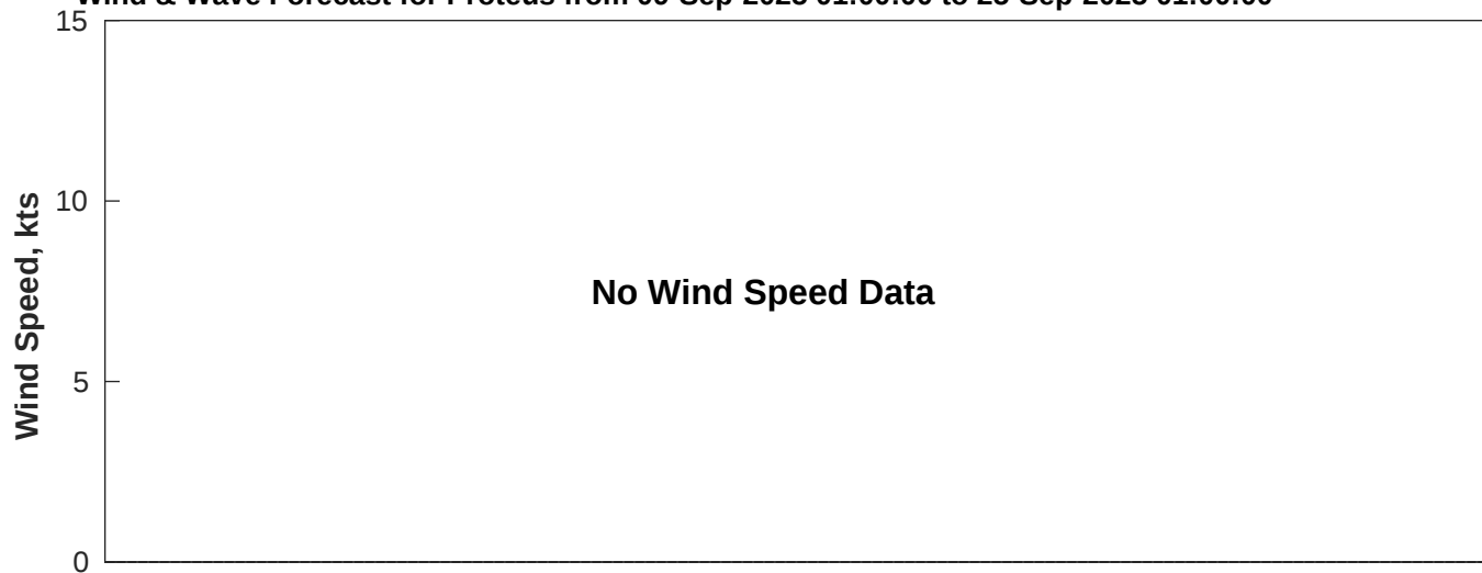
Wind & Wave Forecast for Proteus from 09-Sep-2025 01:00:00 to 25-Sep-2025 01:00:00
