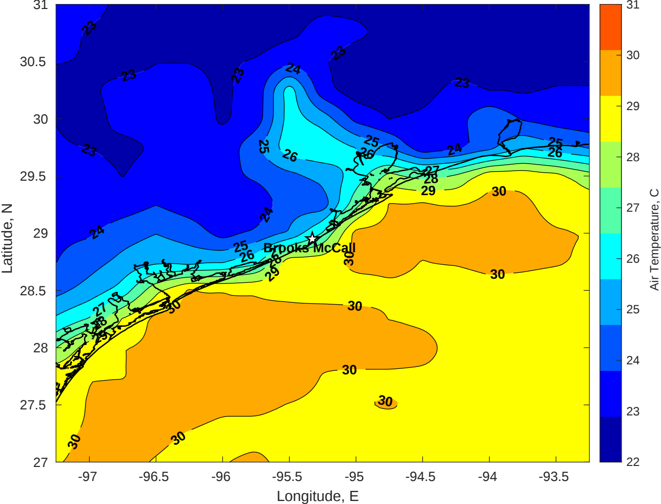
Air Temperature (C) for Brooks McCall at 09-Sep-2025
