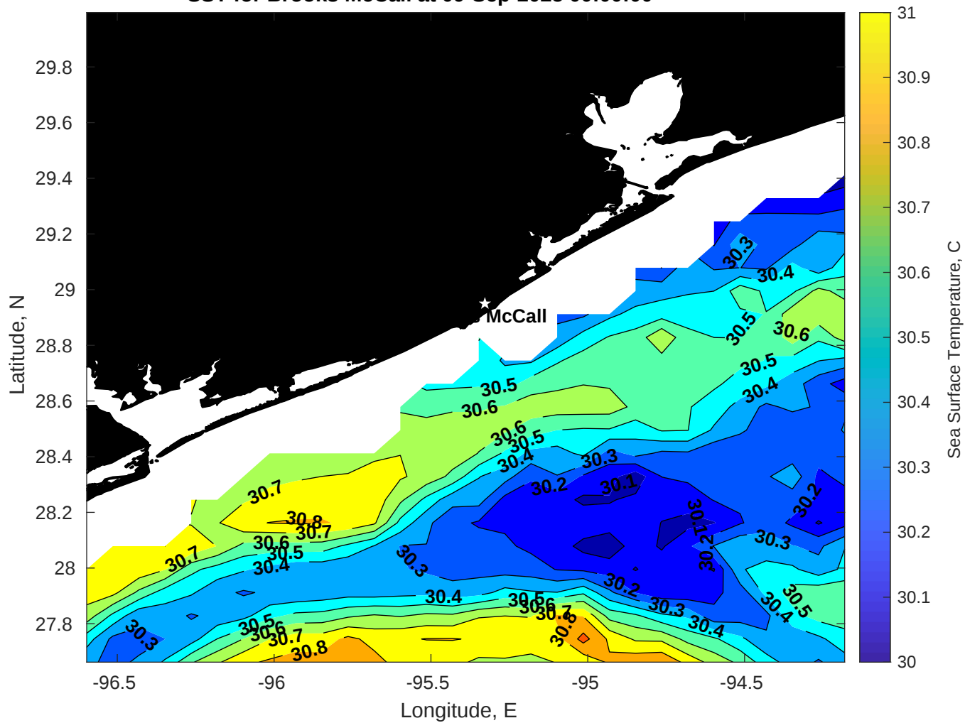
SST for Brooks McCall at 09-Sep-2025 00:00:00
