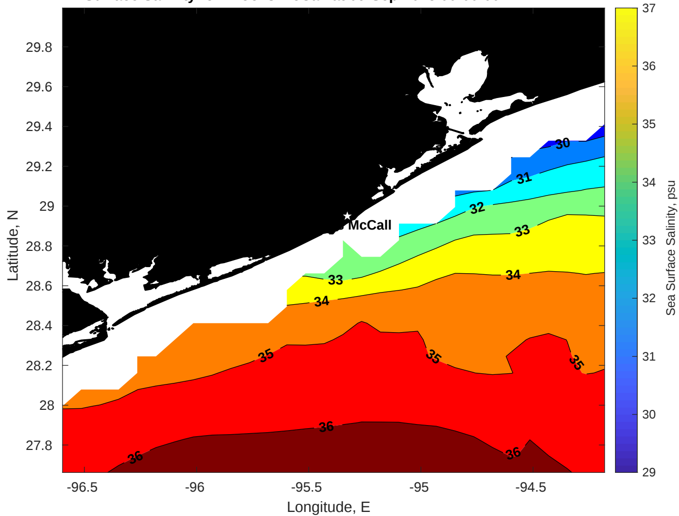
Surface Salinity for Brooks McCall at 09-Sep-2025 00:00:00
