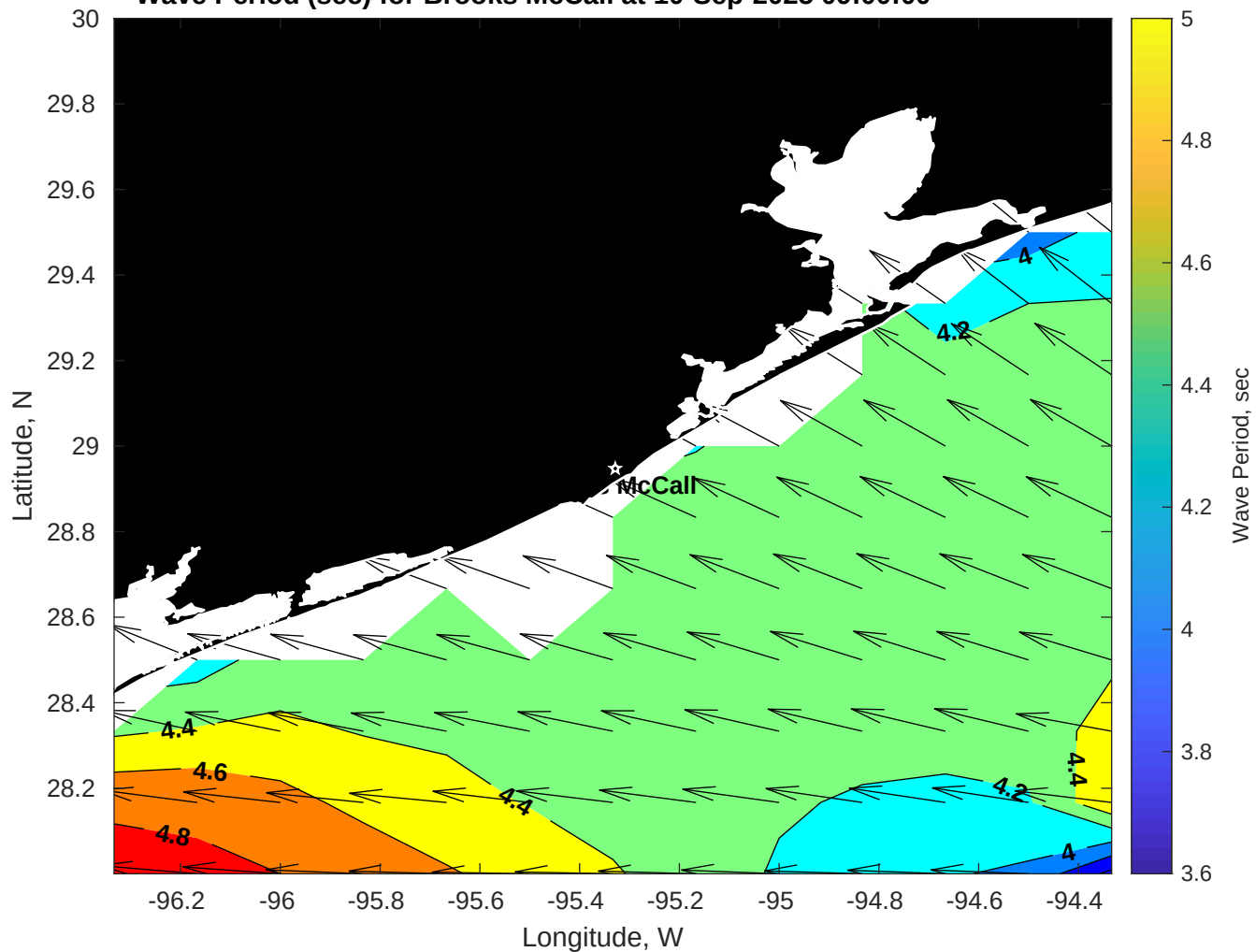
Wave Period (sec) for Brooks McCall at 10-Sep-2025 09:00:00
