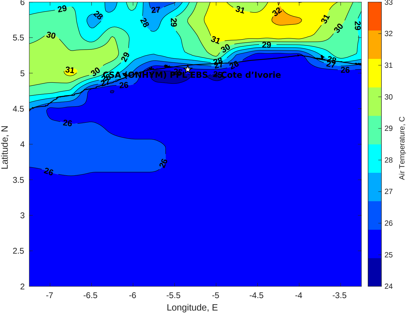
Air Temperature (C) for CSA (ONHYM) PPL EBS - Cote d'Ivoire at 09-Sep-2025
