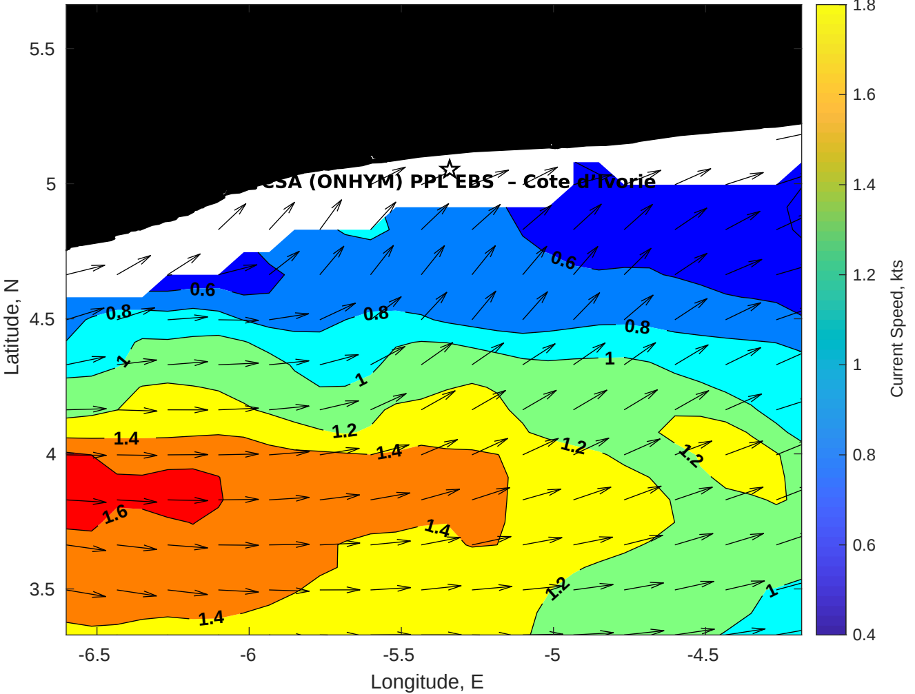
Surface Currents for CSA (ONHYM) PPL EBS - Cote d'Ivoire at 09-Sep-2025 00:00:00
