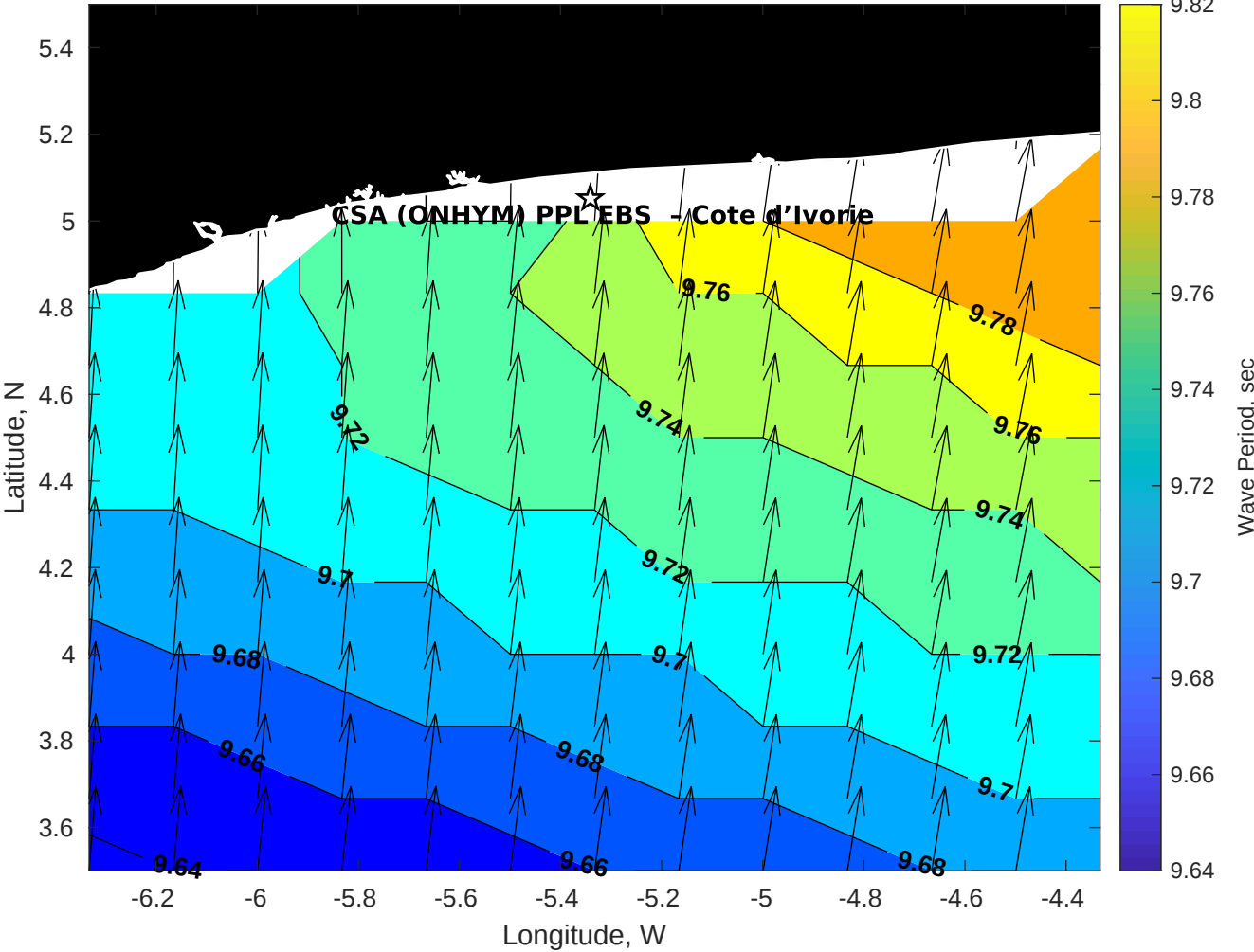
Wave Period (sec) for CSA (ONHYM) PPL EBS - Cote d'Ivoire at 10-Sep-2025 09:00:00
