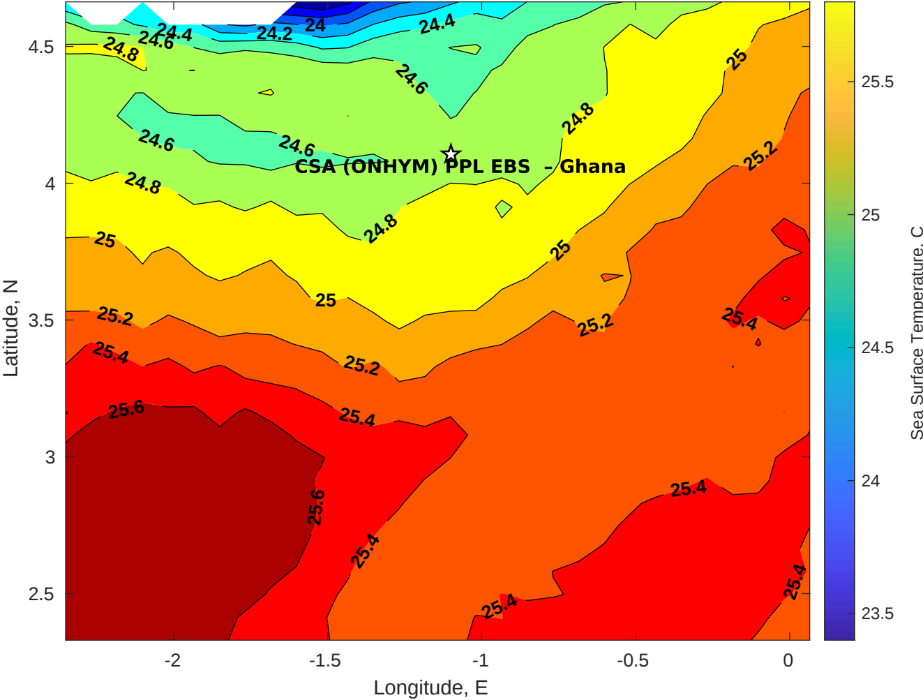
SST for CSA (ONHYM) PPL EBS - Ghana at 09-Sep-2025 00:00:00
