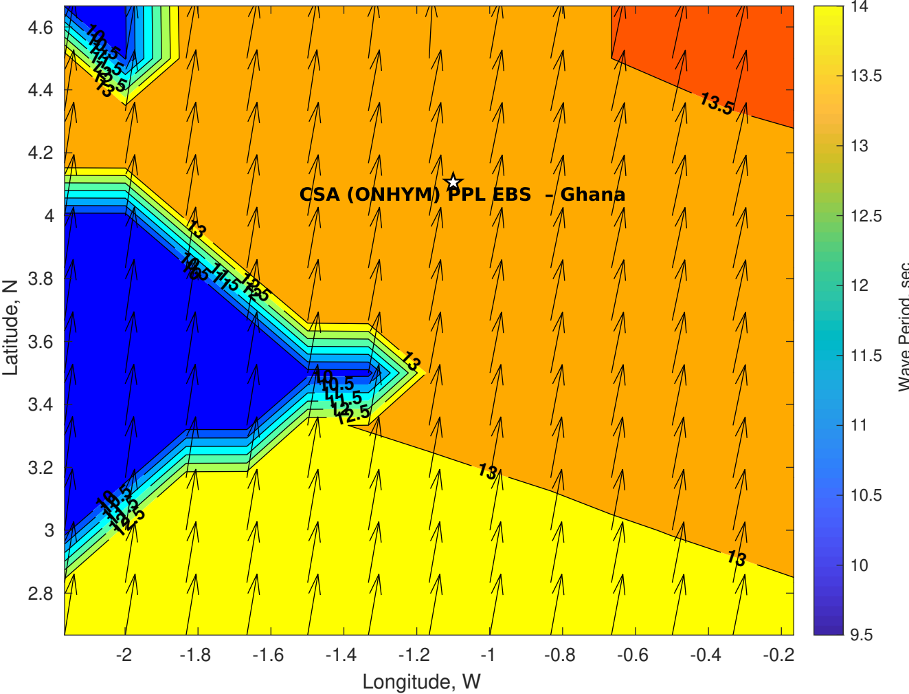
Wave Period (sec) for CSA (ONHYM) PPL EBS - Ghana at 10-Sep-2025 09:00:00
