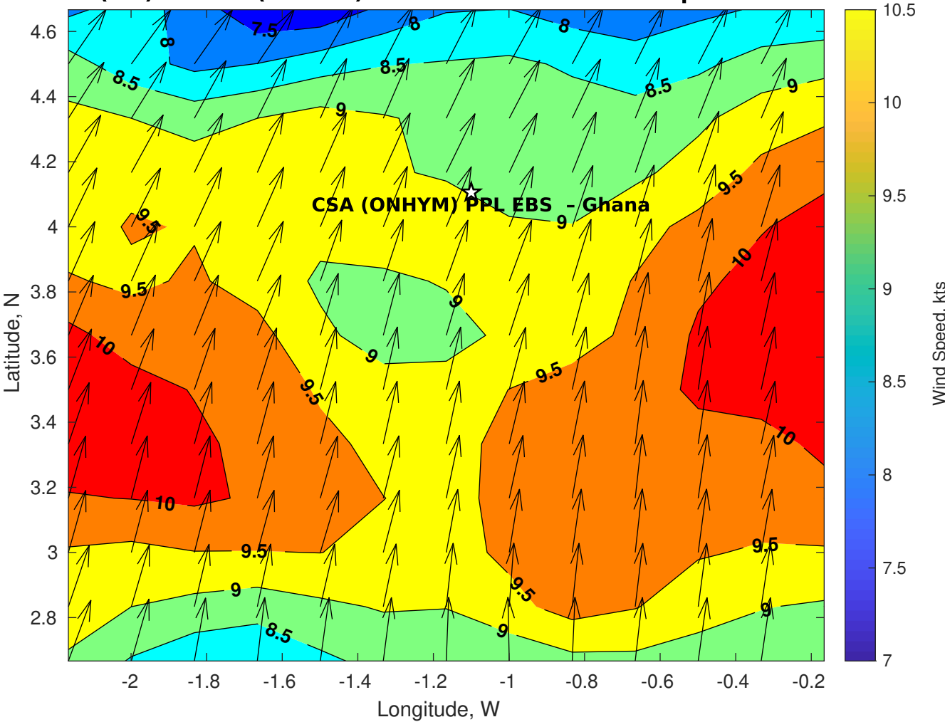
Winds (kts) for CSA (ONHYM) PPL EBS - Ghana at 10-Sep-2025 09:00:00
