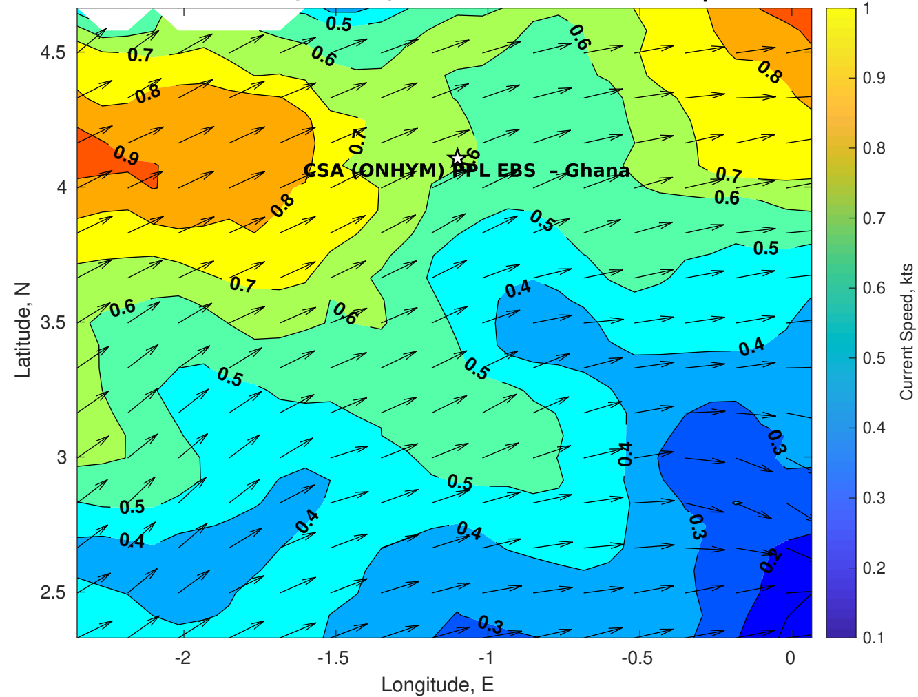
Surface Currents for CSA (ONHYM) PPL EBS - Ghana at 09-Sep-2025 00:00:00
