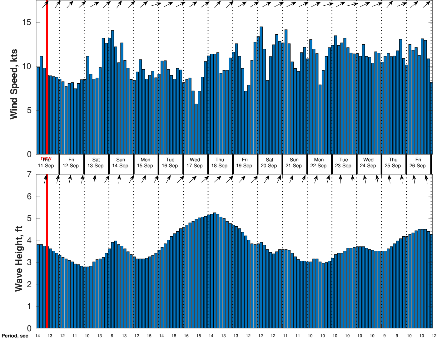
Wind & Wave Forecast for CSA (ONHYM) PPL EBS - Ghana from 10-Sep-2025 02:00:00 to 26-Sep-2025 02:00:00
