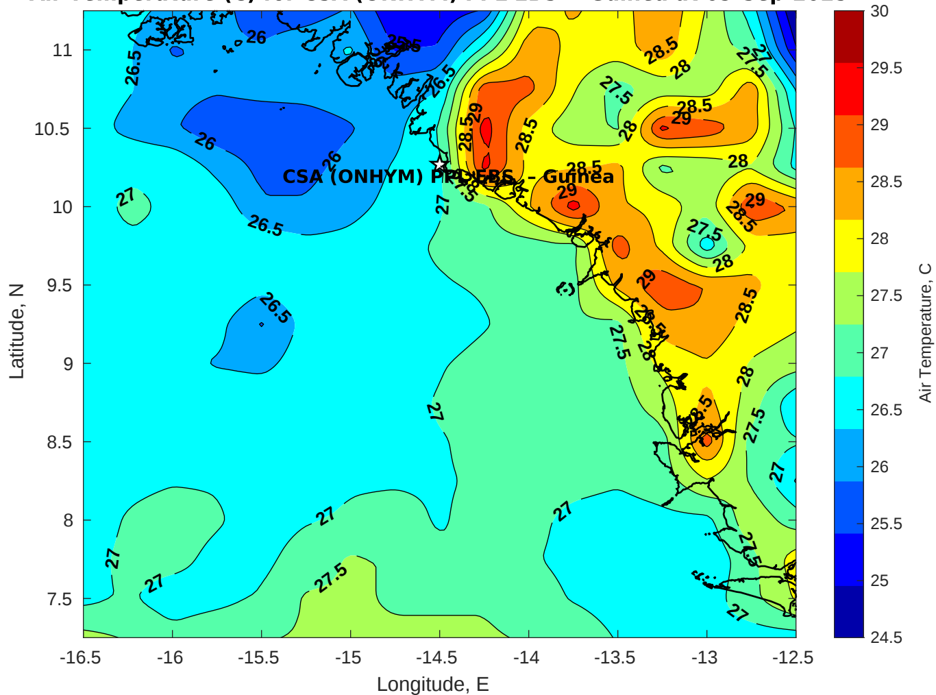
Air Temperature (C) for CSA (ONHYM) PPL EBS - Guinea at 09-Sep-2025
