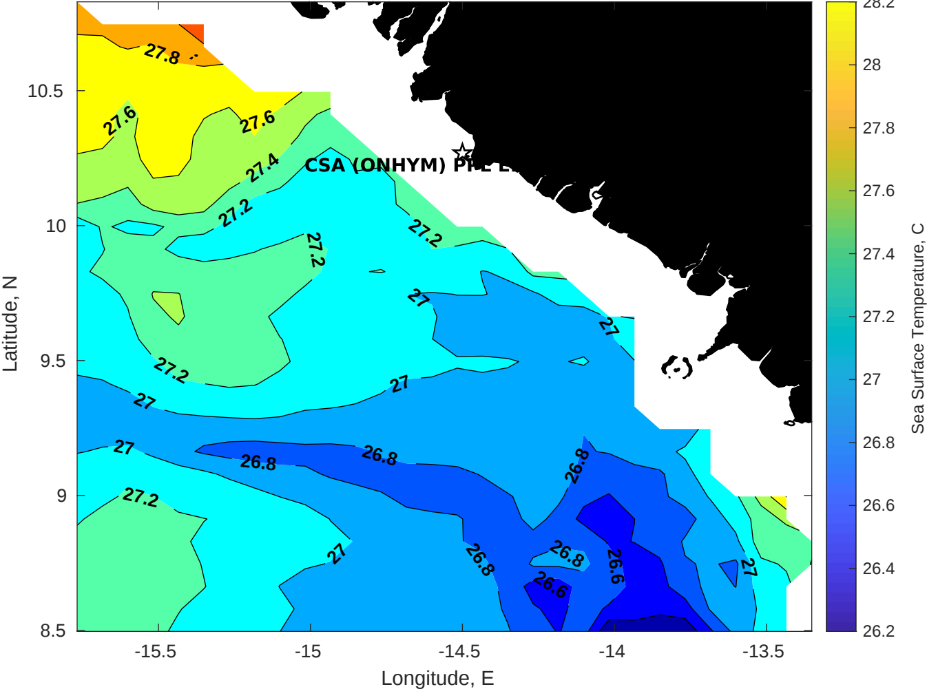
SST for CSA (ONHYM) PPL EBS - Guinea at 09-Sep-2025 00:00:00
